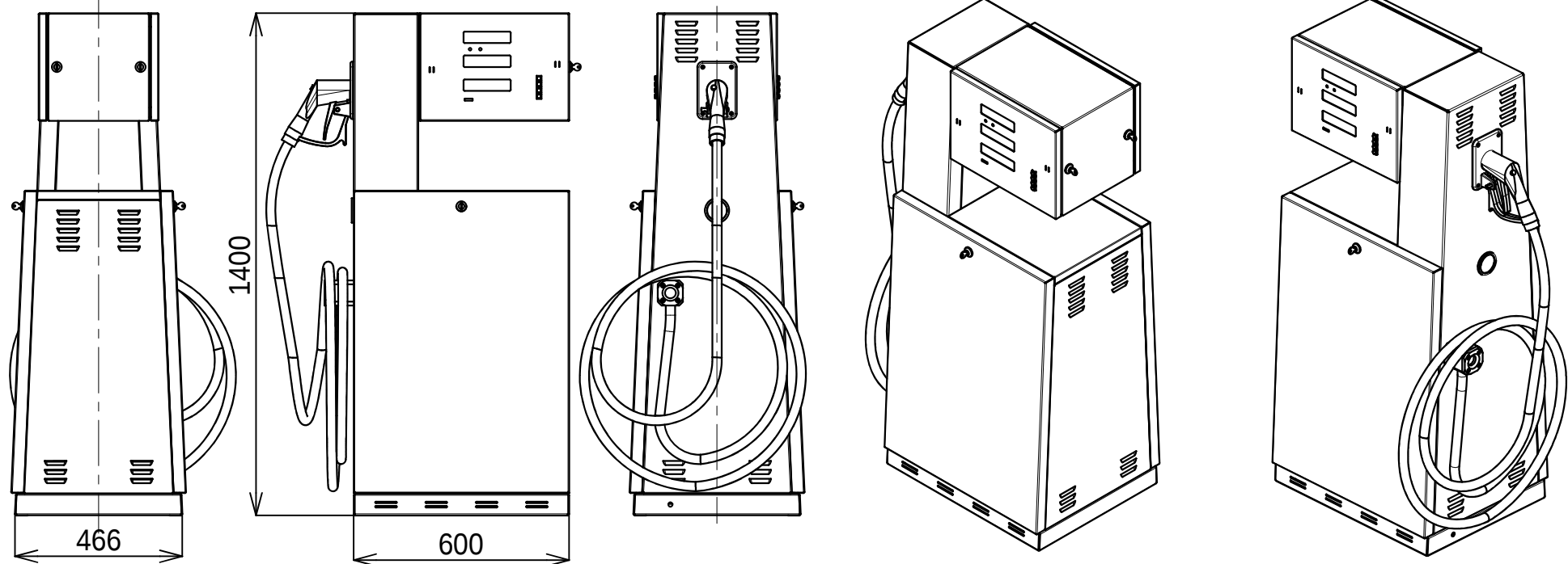
BMP511.SD/LPG
