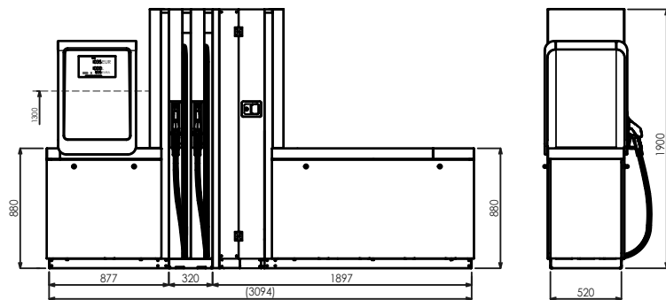
BM4022.OWR+MOD4011.OWR/AdB/T250
