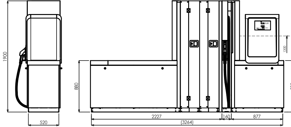
BMP4011.OWL+MOD4012.OWL/AdB/T250
