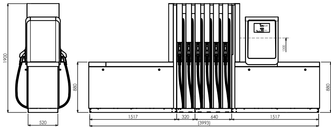
BMP4048.OWD+MOD4014.OWD/AdB-NoHeat/T250
