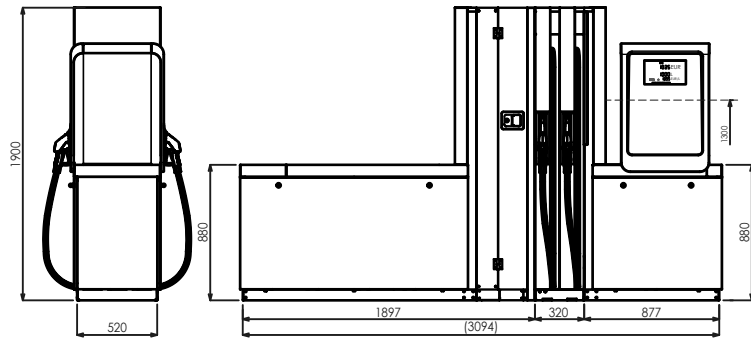
BMP4024.OWD+MOD4012.OWD/AdB/T250
