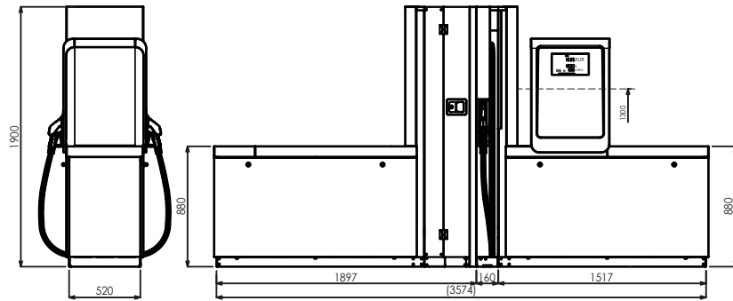
BMP4012.OWD/UH/UH+MOD4012.OWD/AdB/T250
