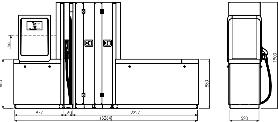
BMP4011.OWR+MOD4012.OWR/AdB/T250
