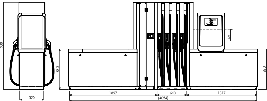
BMP4048.OWD+MOD4012.OWD/AdB/T250
