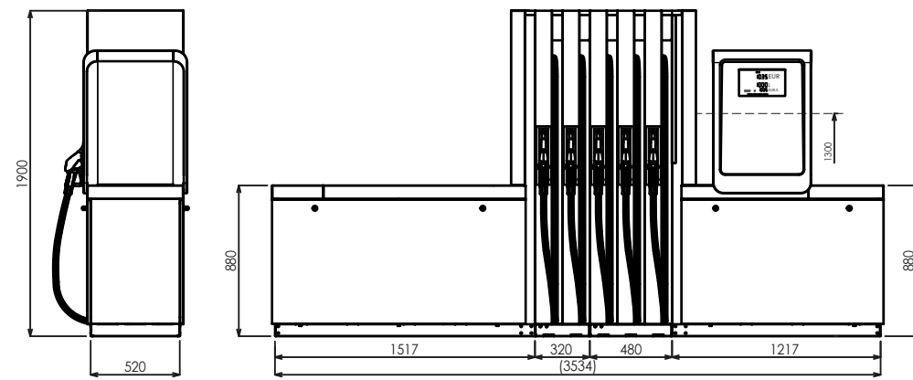
BMP4033.OWL+MOD4012.OWL/AdB-NoHeat/T250
