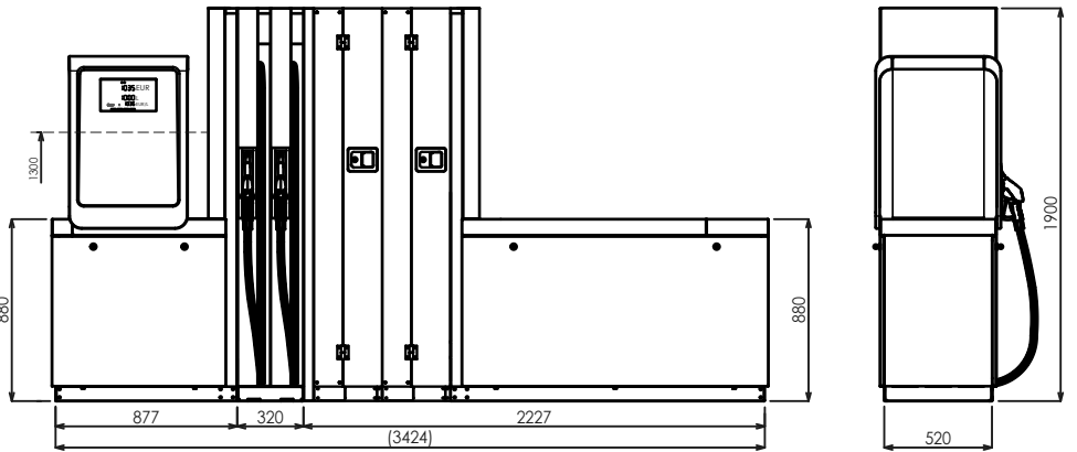
BM4022.OWR+MOD4012.OWR/AdB/T250
