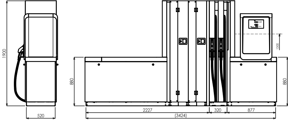
BMP4022.OWL+MOD4012.OWL/AdB/T250
