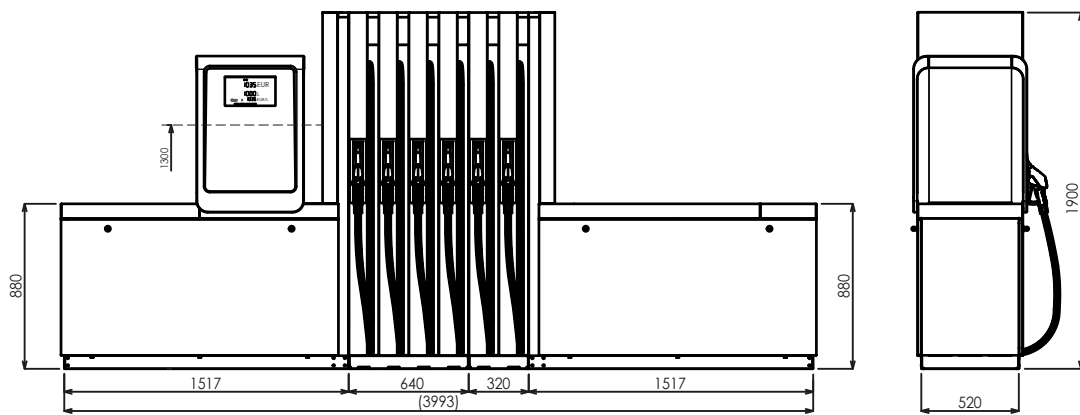
BM4044.OWR+MOD4012.OWR/AdB-NoHeat/T250
