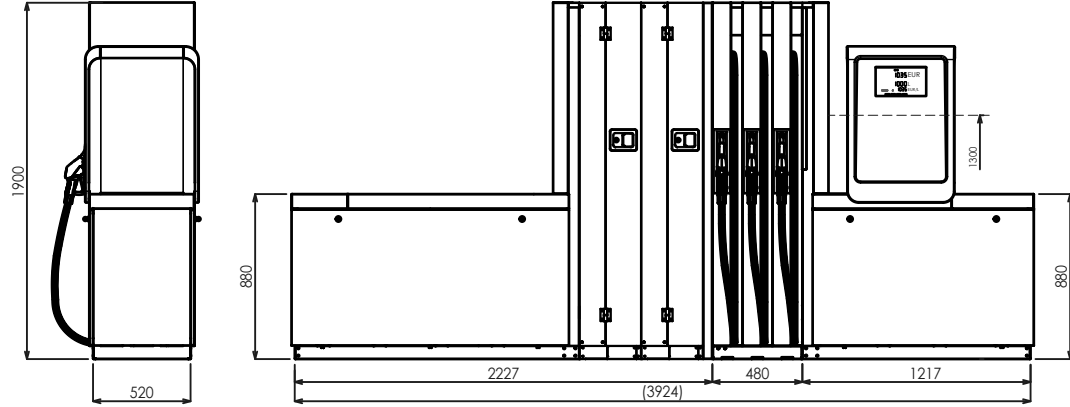
BMP4033.OWL+MOD4012.OWL/AdB/T250
