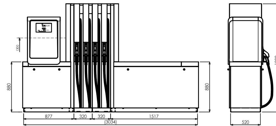
BM4022.OWR+MOD4012.OWR/AdB-NoHeat/T250
