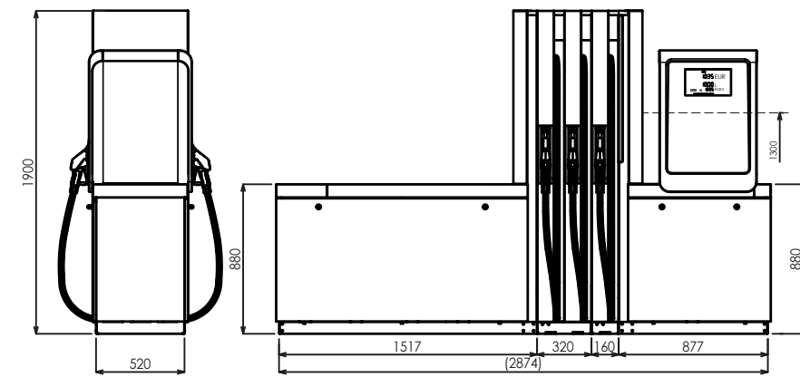
BMP4012.OWD+MOD4014.OWD/AdB-NoHeat/T250
