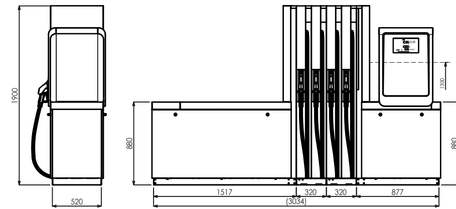
BMP4022.OWL+MOD4012.OWL/AdB-NoHeat/T250
