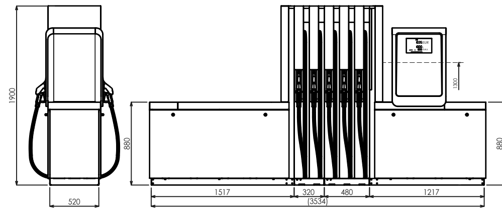
BMP4036.OWD+MOD4014.OWD/AdB-NoHeat/T250
