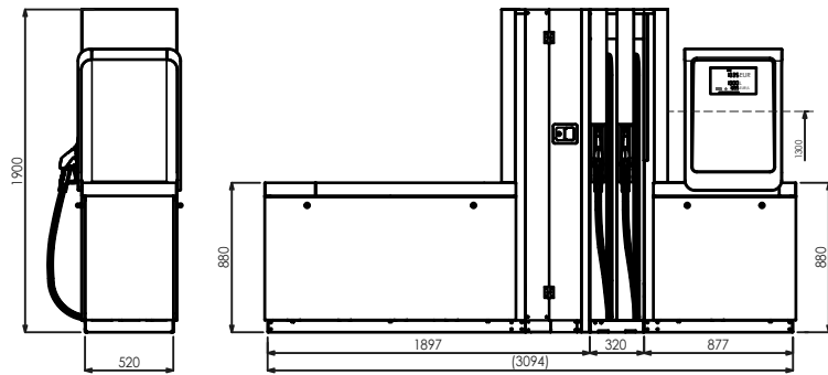
BMP4022.OWL+MOD4011.OWL/AdB/T250
