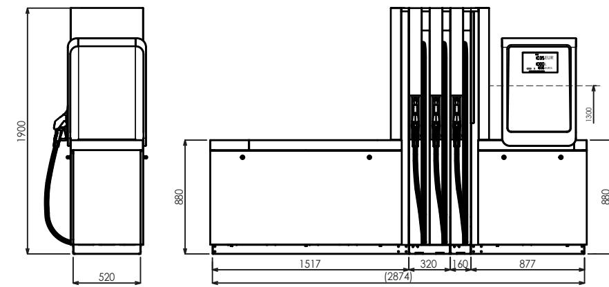
BMP4011.OWL+MOD4012.OWL/AdB-NoHeat/T250
