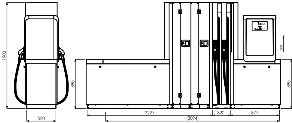
BMP4024.OWD+MOD4014.OWD/AdB/T250
