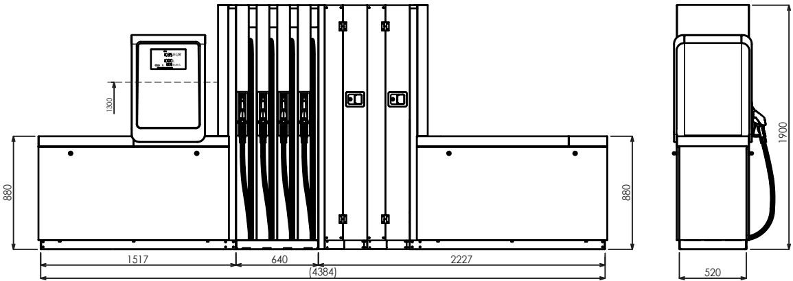
BM4044.OWR+MOD4012.OWR/AdB/T250
