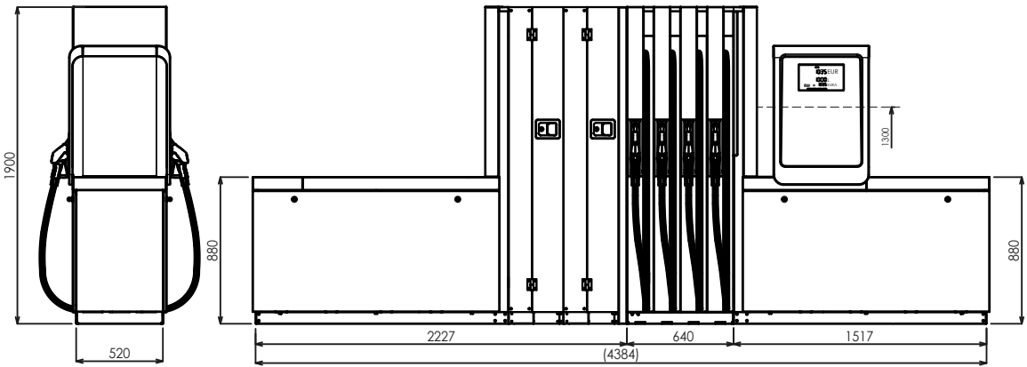
BMP4048.OWD+MOD4014.OWD/AdB/T250
