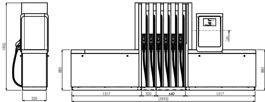
BMP4044.OWL+MOD4012.OWL/AdB-NoHeat/T250
