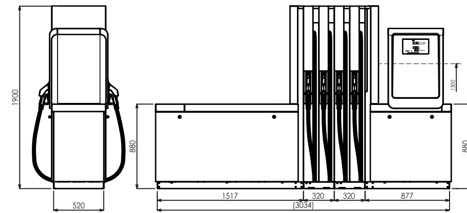
BMP4024.OWD+MOD4014.OWD/AdB-NoHeat/T250
