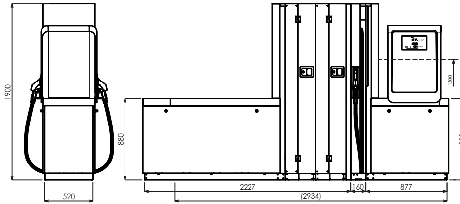
BMP4012.OWD+MOD4014.OWD/AdB/T250
