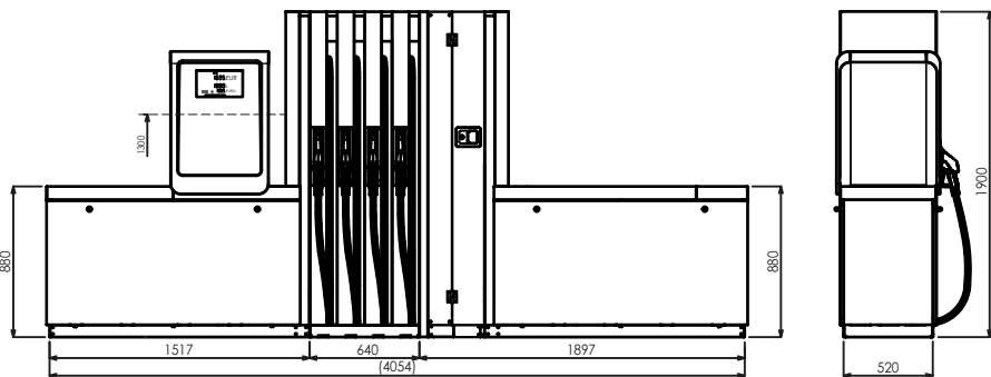
BM4044.OWR+MOD4011.OWR/AdB/T250
