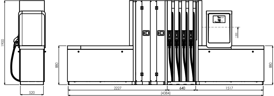
BMP4044.OWL+MOD4012.OWL/AdB/T250
