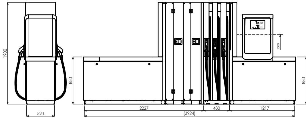
BMP4036.OWD+MOD4014.OWD/AdB/T250
