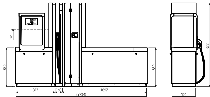
BMP4011.OWR+MOD4011.OWR/AdB/T250
