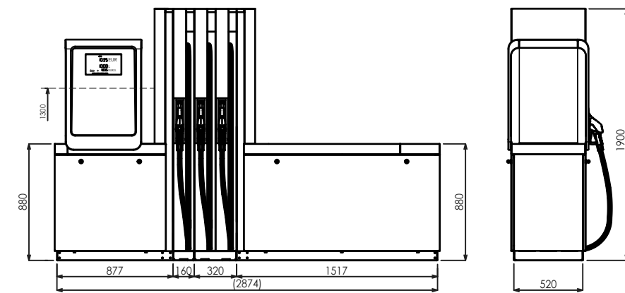
BMP4011.OWR+MOD4012.OWR/AdB-NoHeat/T250
