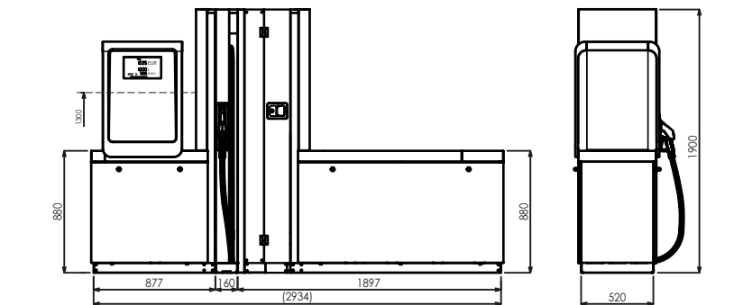
BMP4021.OWR/UH+MOD4011.OWR/AdB/T250
