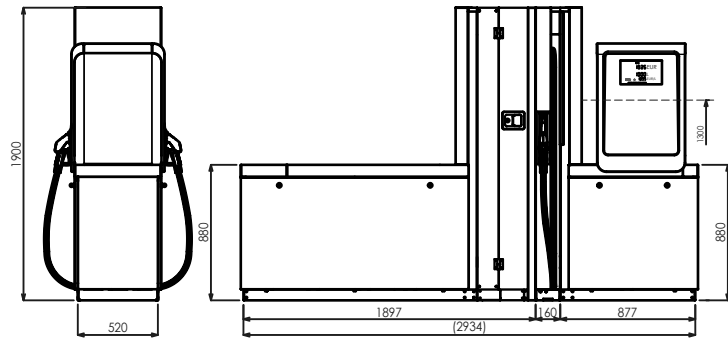
BMP4012.OWD+MOD4012.OWD/AdB/T250
