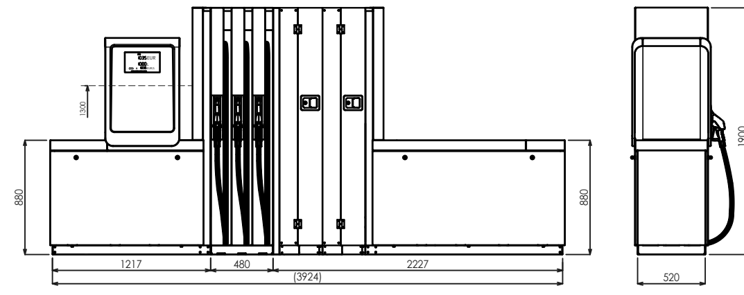
BM4033.OWR+MOD4012.OWR/AdB-NoHeat/T250
