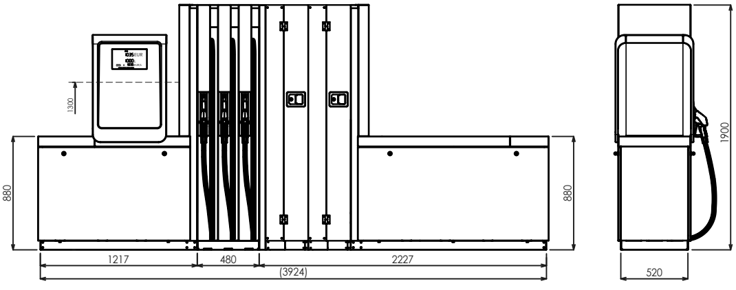
BM4033.OWR+MOD4012.OWR/AdB/T250
