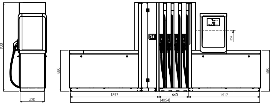
BMP4044.OWL+MOD4011.OWL/AdB/T250
