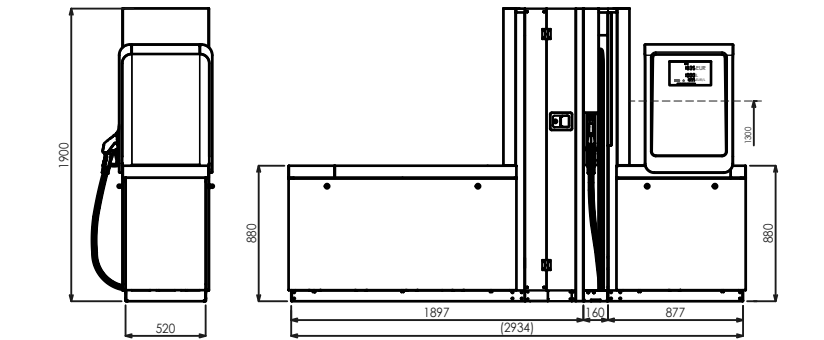
BMP4021.OWL/UH+MOD4011.OWL/AdB/T250
