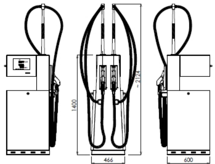
BMP512.SR/AdB-HS
