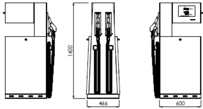
BMP512.SL/AdB
