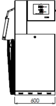
BMP511.SL/AdB/HT
