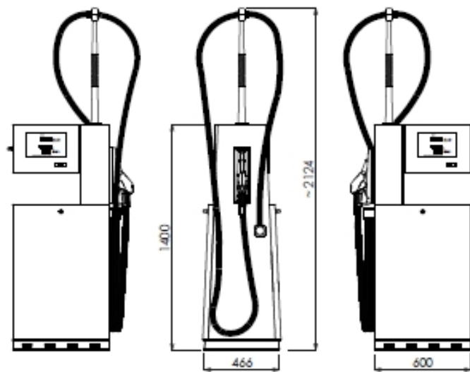
BMP511.SD/AdB-HS
