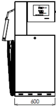
BMP511.SD/AdB/HT
