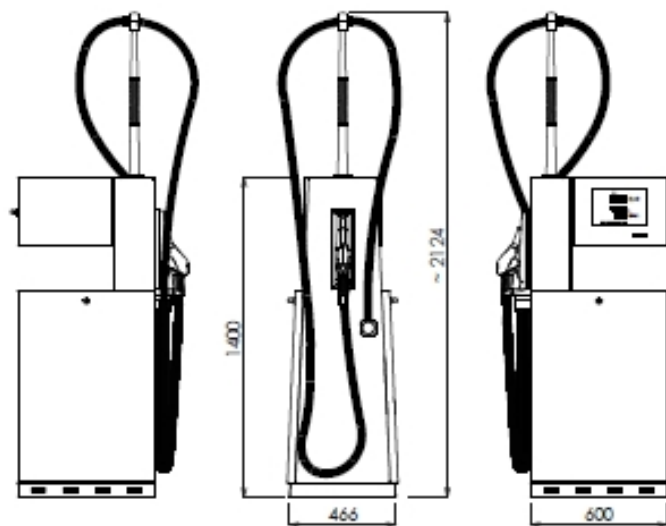
BMP511.SL/AdB-HS
