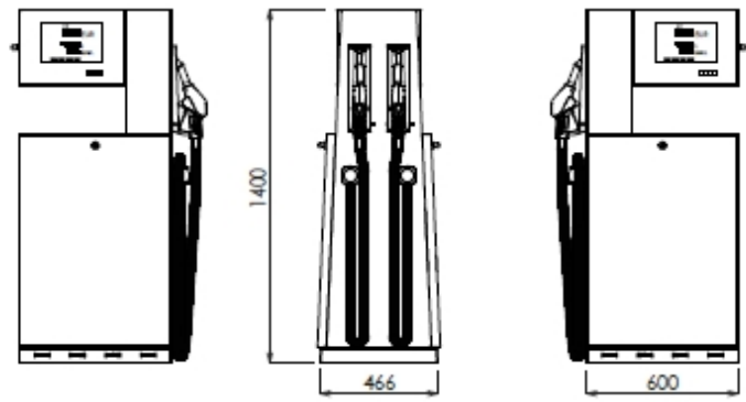
BMP512.SD/AdB
