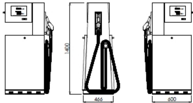
BMP511.SD/AdB
