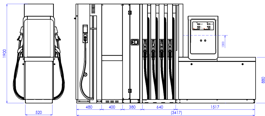
BMP4048.OWD+MOD4012.OWD/AdB+MOD40x2.OWD/CNG
