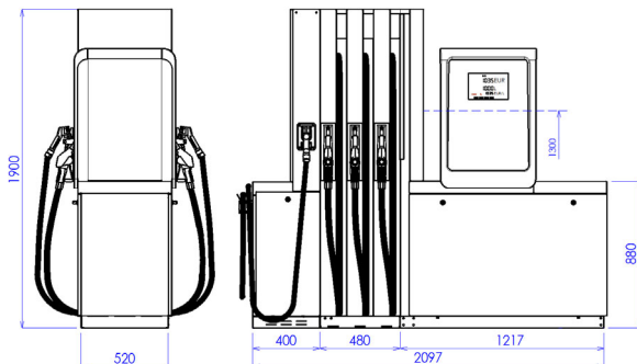
BMP4036.OWD+MOD4012.OWD/LPG
