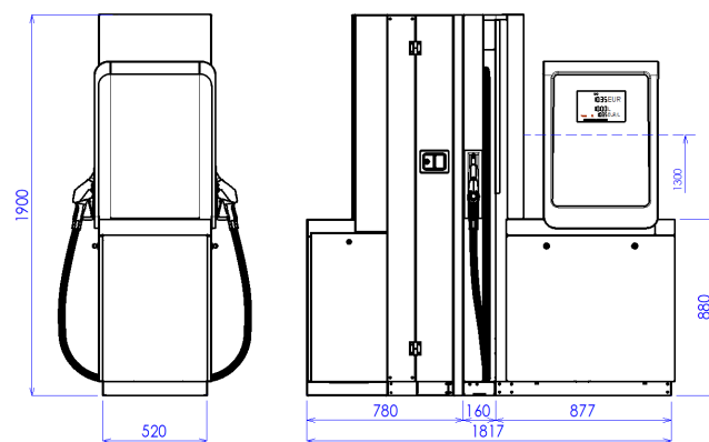
BMP4012.OWD+MOD4012.OWD/AdB
