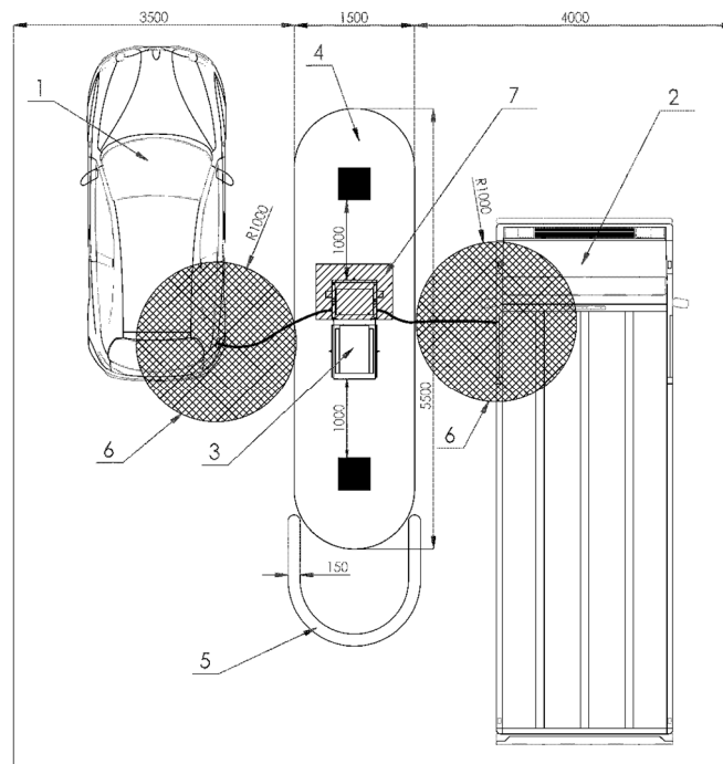
Figure 68 – Example of the CNG dispenser location at the fuel station
