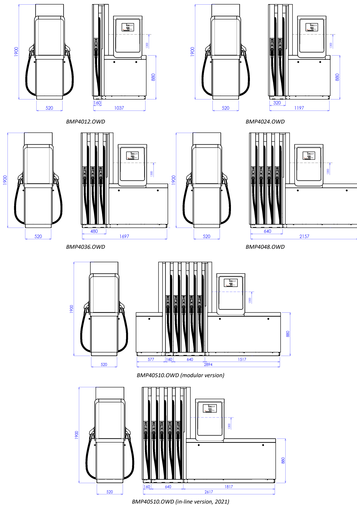
Figure 28 - Overview of standard OCEAN TOWER models
