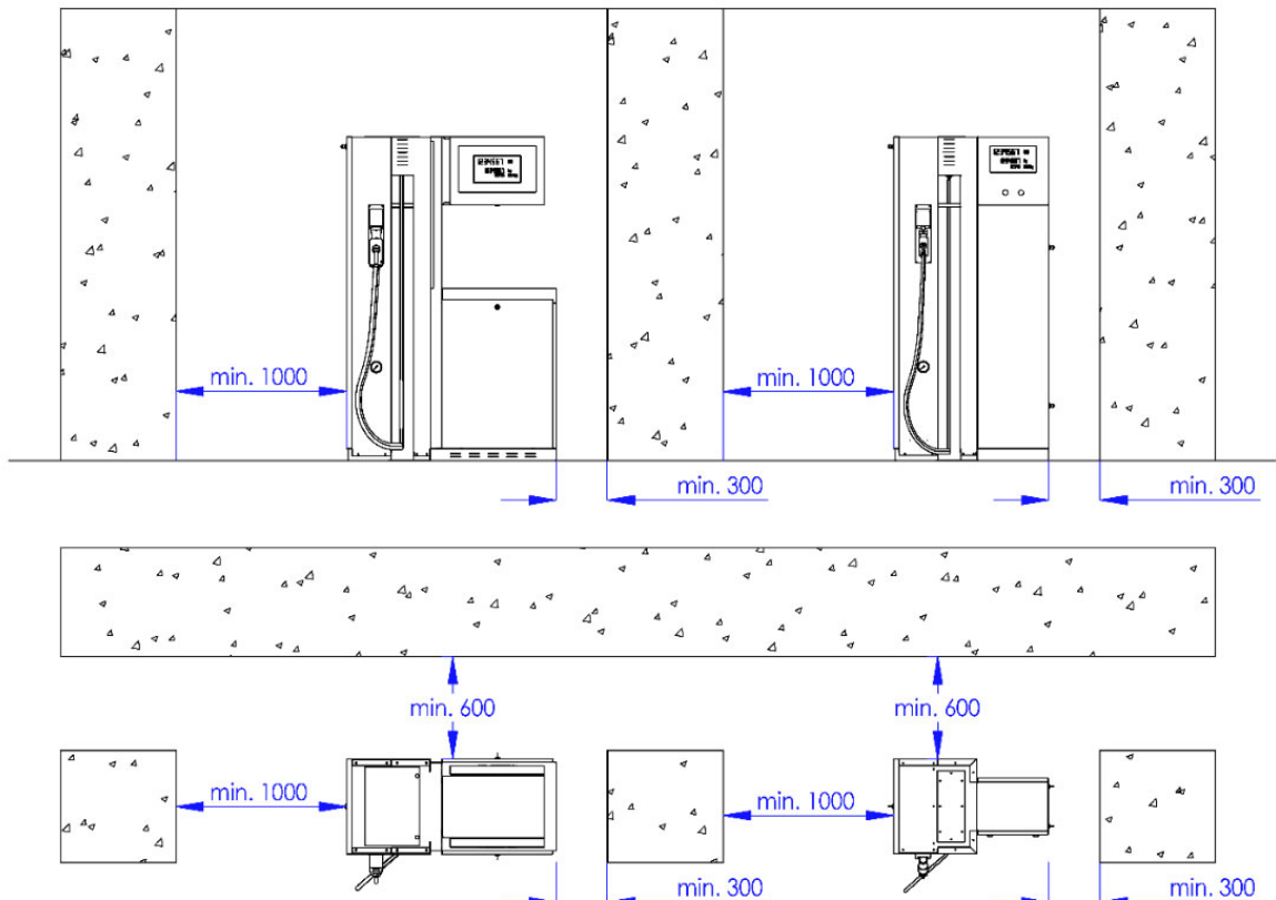
Figure 67 – Minimum recommended separation distance of the dispenser from a fixed obstacle
