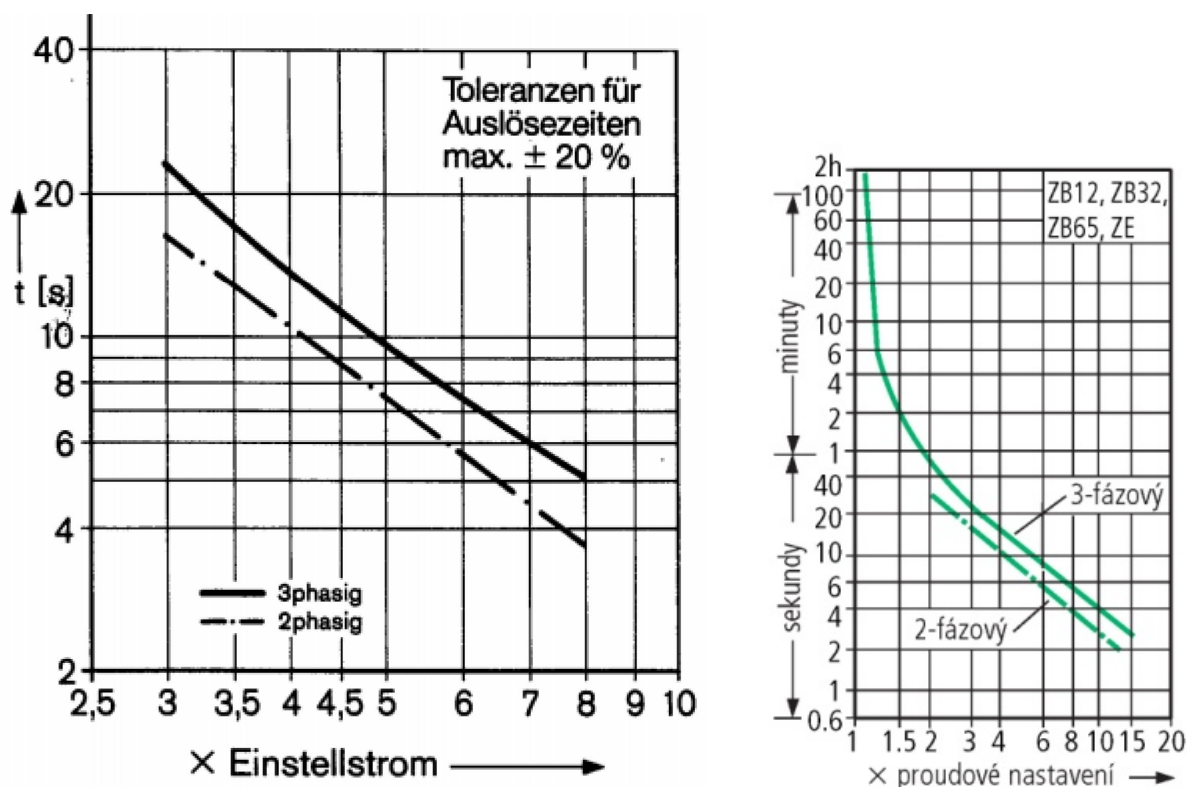
Picture 74 – Access characteristics of the motor current protection, type ZE
