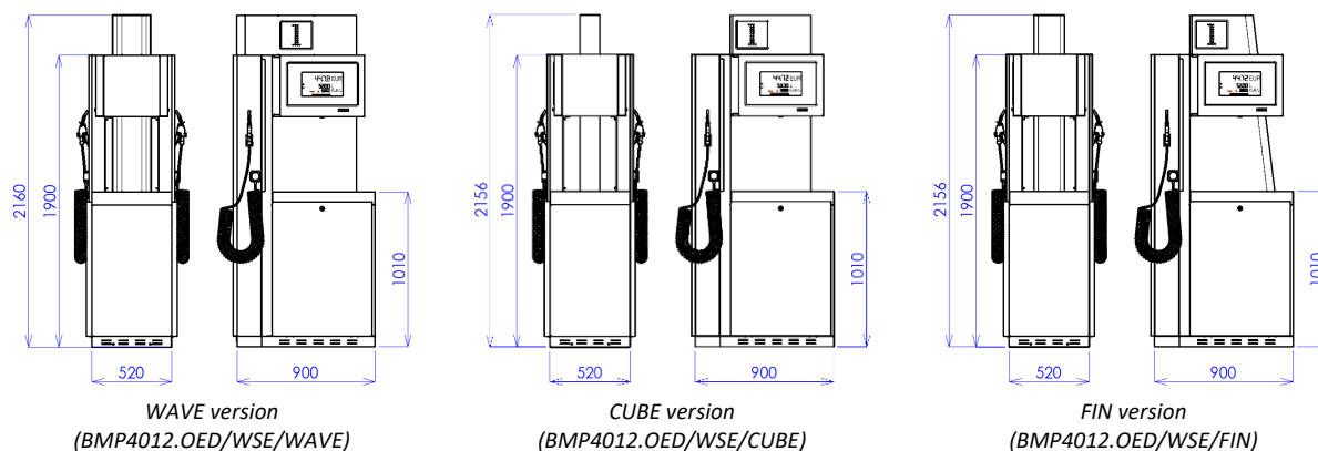
Figure 21 - Design variants of OCEAN EURO WSE dispensers
