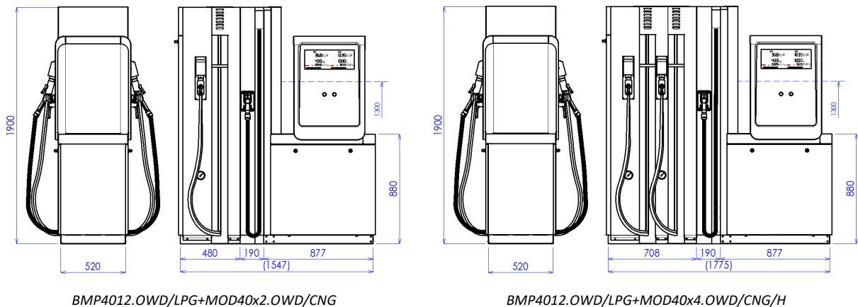
Figure 49 -Overview of OCEAN TOWER COMBI LPG dispensers with CNG module, x=1,2,3 is number of CNG inlets
