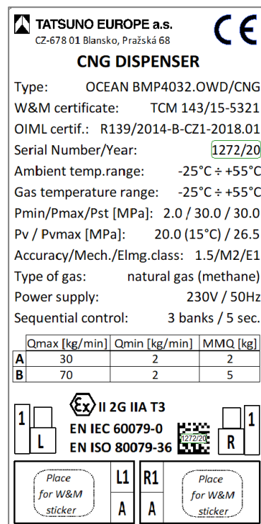
Figure 63 - Nameplate of two-hose CNG dispenser
