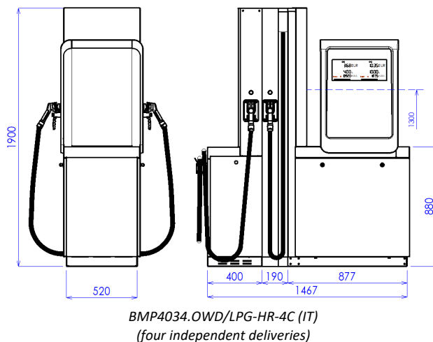
Picture 31 – Special model of the dispenser OCEAN TOWER LPG with two hose retractors and two free hanging hoses (for long distance nozzle reach)
