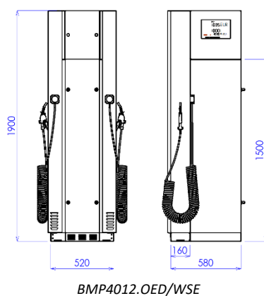
Picture 26 - Standard model of OCEAN SMART WSE dispenser
