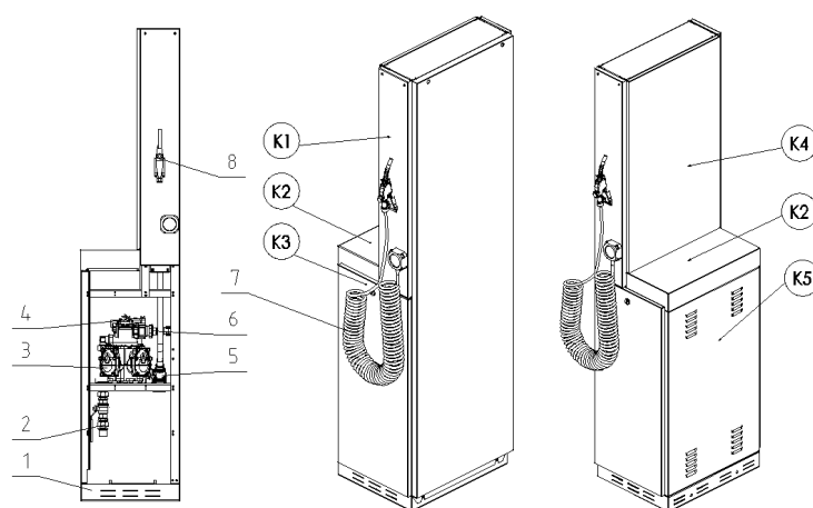
Figure 54 - Basic parts of the WSE dispensing module and its cover
