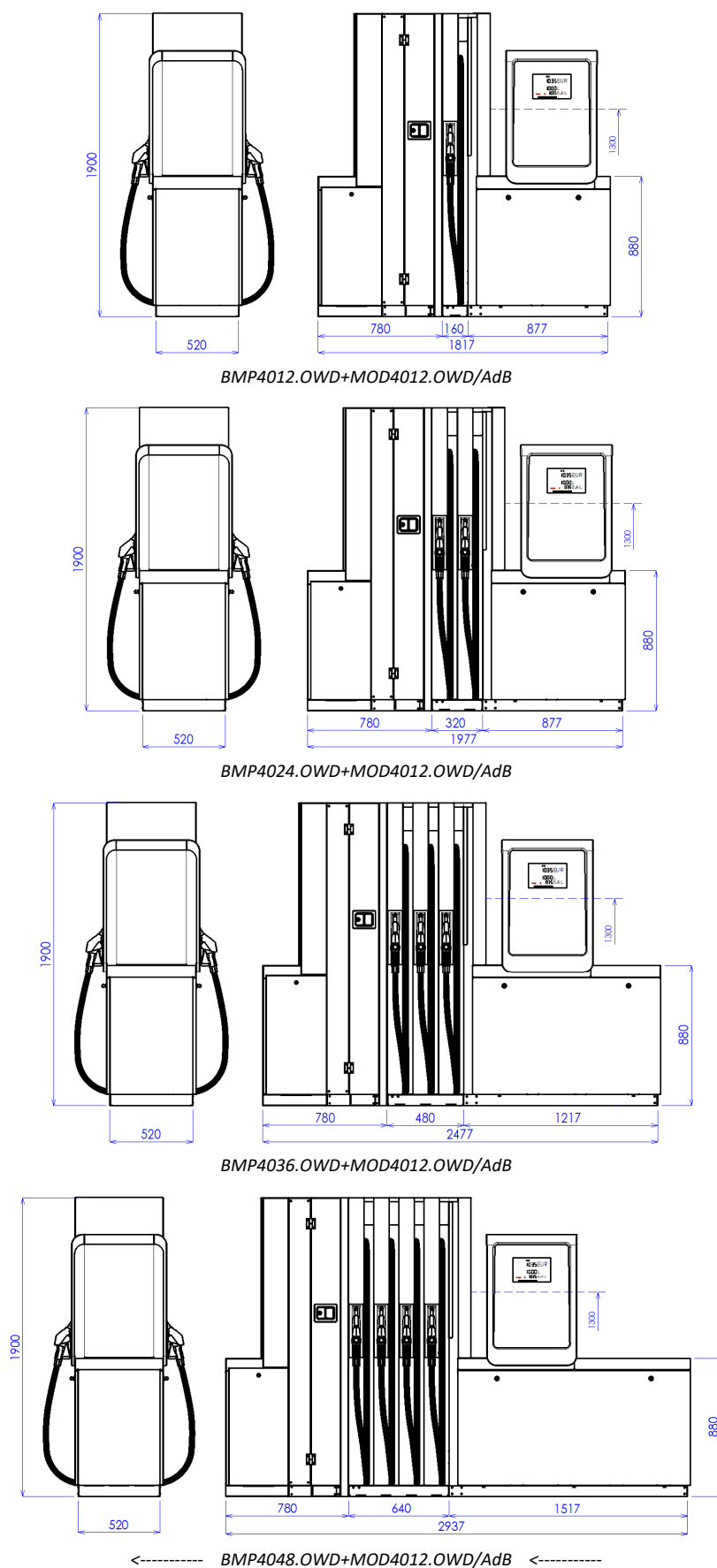
Figure 41 – Overview of standard OCEAN TOWER COMBI ADB dispensers with heating of the AdBlue module
