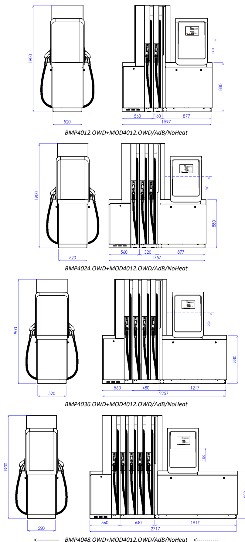
Figure 42 – Overview of OCEAN TOWER COMBI ADB dispensers with AdBlue module without heating (for temperatures from 0°C to 40°C).
