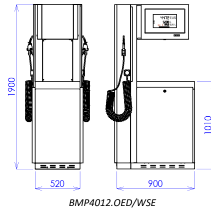
Figure 22 - Overview of standard OCEAN EURO WSE dispensers
