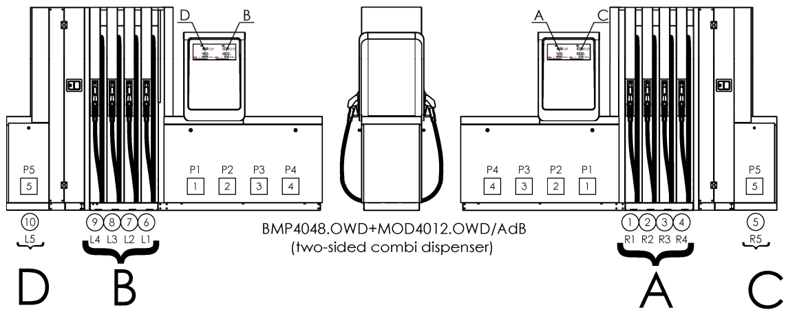
Picture 80 – Example of a combined dispenser with four filling points A, B, C and D (four simultaneous deliveries, four main displays; ①, ②, ③ ... - nozzle position in electronic counter)
