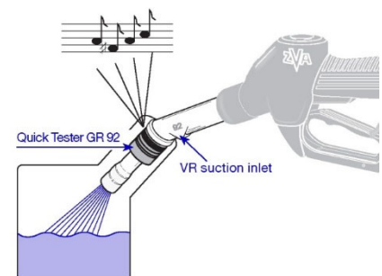
Picture 83 – Functional recuperation test with Quick Tester GR 92 adapter
