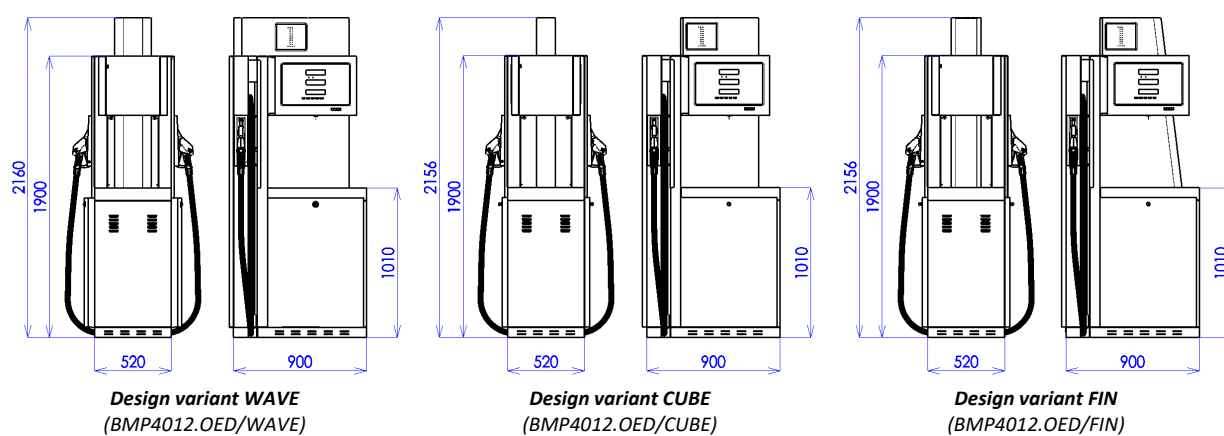
Figure 14 - Design variants of OCEAN EURO dispensers
