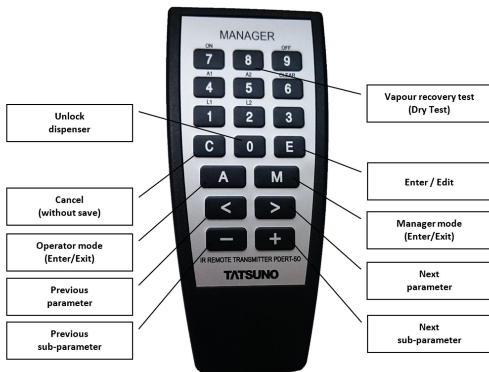
Figure 78 – Description of keys of the PDERT-50 remote controller
