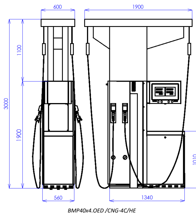
Figure 25 – Model of OCEAN EURO CNG dispenser with hose extender (HE = hose extender)
