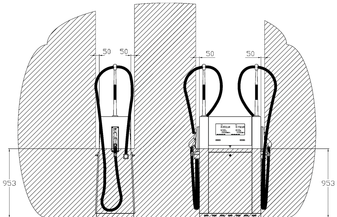
Picture 70 – Example of possible placement of the AdBlue® dispenser in zone 2
