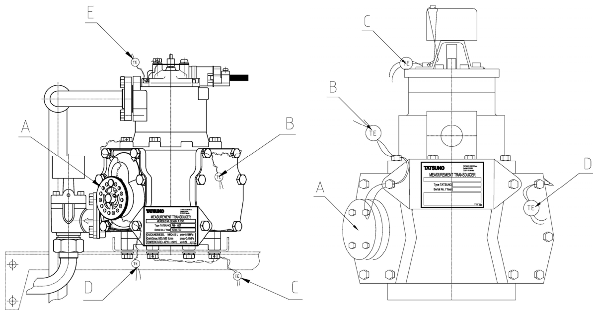
Figure 90 – Piston meters of fuel (type FM-1007) and LPG (type MP-02524 and FM-1029), A=calibration wheel
