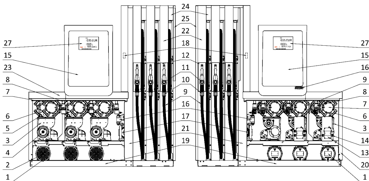
Picture 50 - Basic parts of the OCEAN TOWER dispenser
