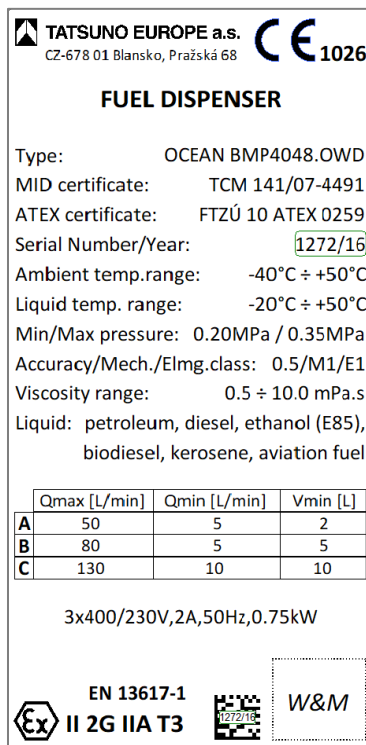
Figure 57 - Nameplate of the multi-hose gasoline/diesel combined
