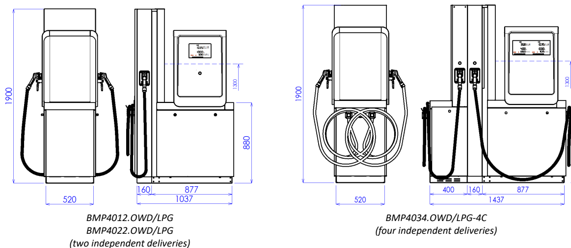
Figure 29 – Overview of standard OCEAN TOWER LPG dispensers with free hanging hoses
