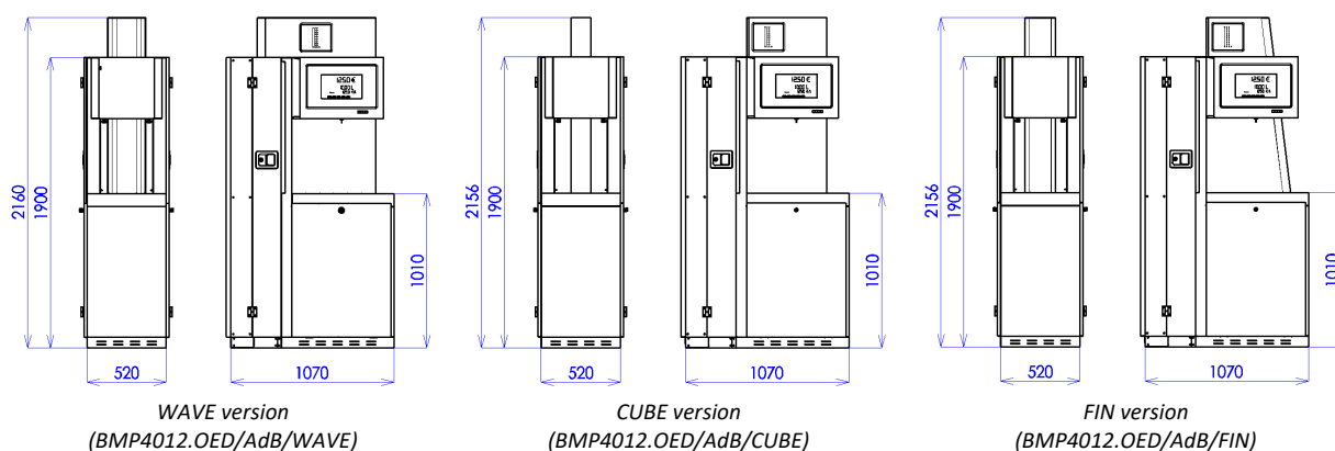
Figure 18 - Design variants of OCEAN EURO ADBLUE® dispensers
