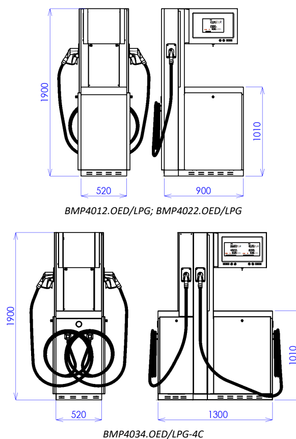
Figure 16 - Overview of standard OCEAN EURO LPG models without hose reels
