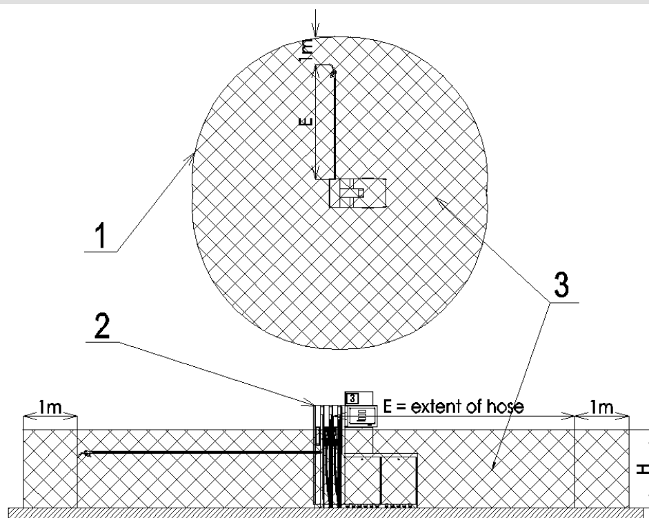
Picture 71 - Spatial restrictions for AdBlue dispensers without ATEX certification
