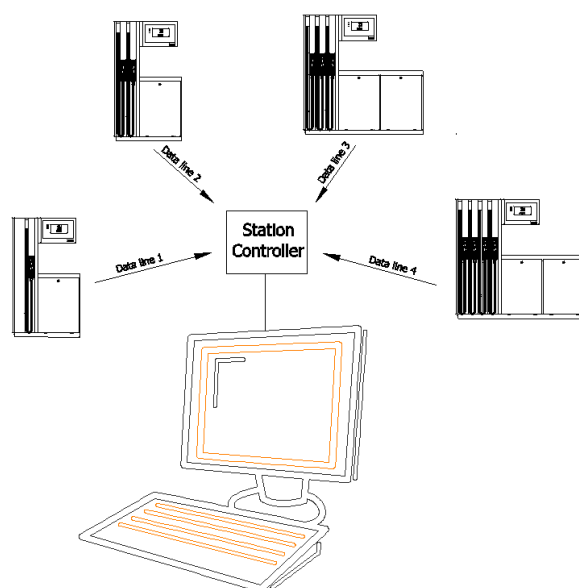
Figure 76 – Radial data line from dispensers
