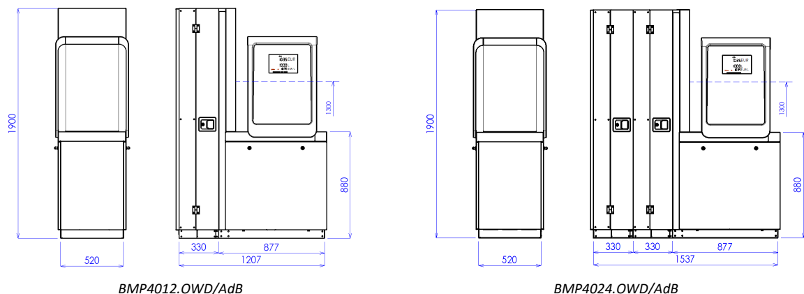
Figure 32 – OCEAN TOWER ADBLUE® standard model with internal heating
