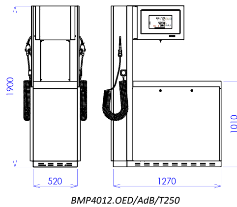
Figure 23 - Model of OCEAN EURO ADBLUE® dispenser with 250L storage tank and pump
