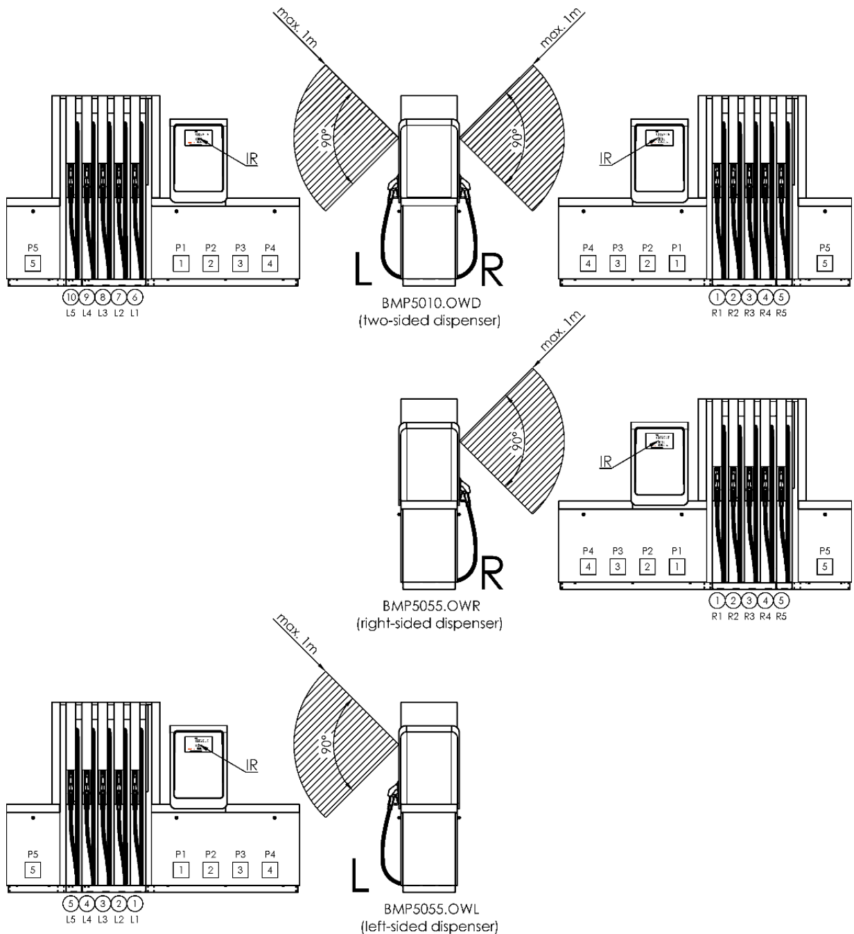
Figure 77 – Range of operation of the remote controller and marking of hoses and products in electronic counter (IR - position of infrared receiver on the display; ①, ②, ③ ... - nozzle position in calculator)
