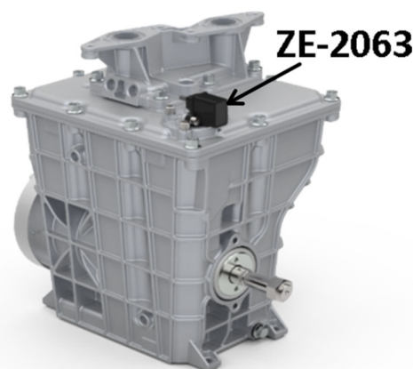
Picture 85 – Pumping monoblock FP-1022 (MVP-X) with air flow sensor ZE-2063
