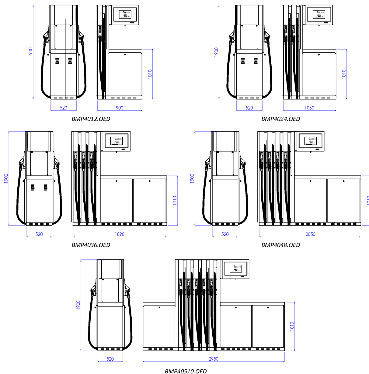
Figure 13 - Overview of standard OCEAN EURO models in basic design
