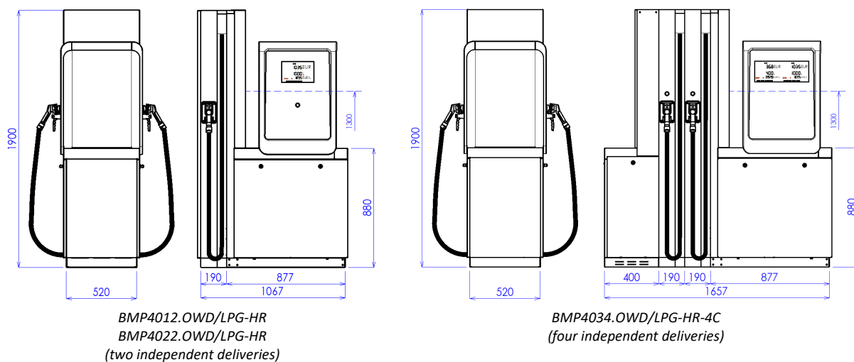
Figure 30 - Overview of standard OCEAN TOWER LPG dispensers with hose reels (-HR)
