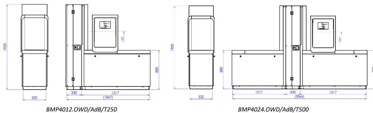
Picture 34 - OCEAN TOWER ADBLUE® dispenser model with internal heating and storage tank 250L or 500L
