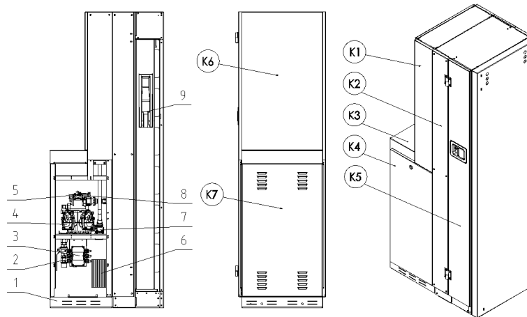
Figure 53 - Basic parts of the AdBlue® dispensing module and its cover
