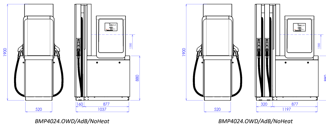
Figure 33 - OCEAN TOWER ADBLUE® dispenser model without internal heating
