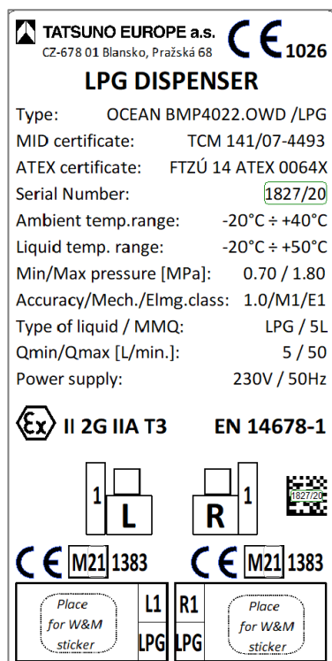
Figure 60 - Nameplate of two-hose LPG dispenser
