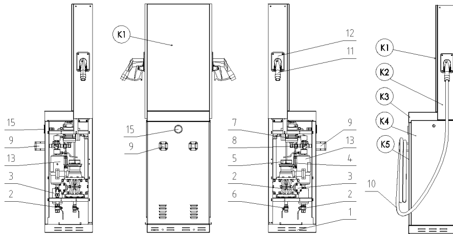
Figure 52 - Basic parts of the LPG dispensing module and its cover
