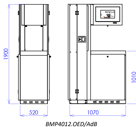
Figure 19 - Overview of standard OCEAN EURO ADBLUE® dispensers
