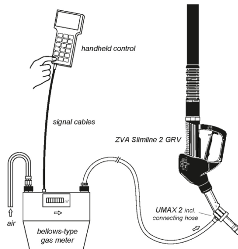
Picture 82 - Connecting the delivery nozzle with an adapter and gas meter
