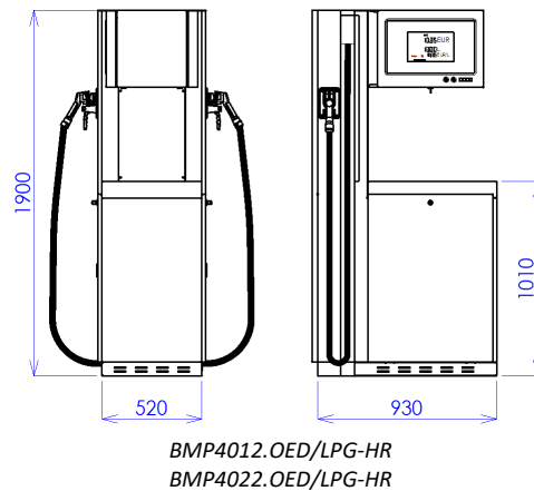
Figure 17 - Overview of standard OCEAN EURO LPG models with delivery hose reels
