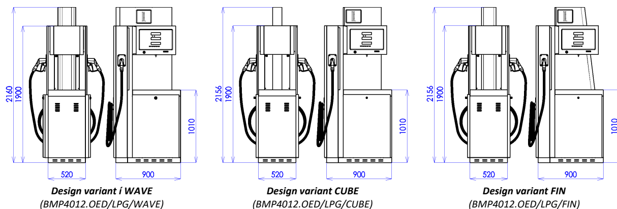
Figure 15 - Design variants of OCEAN EURO LPG dispensers
