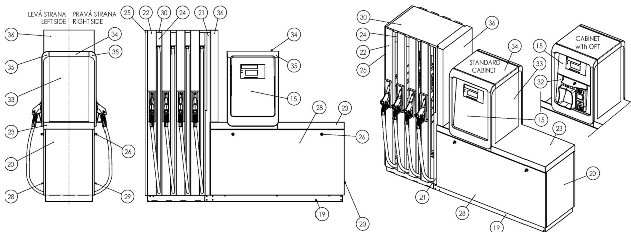
Picture 51 - Covers of the OCEAN TOWER dispenser
