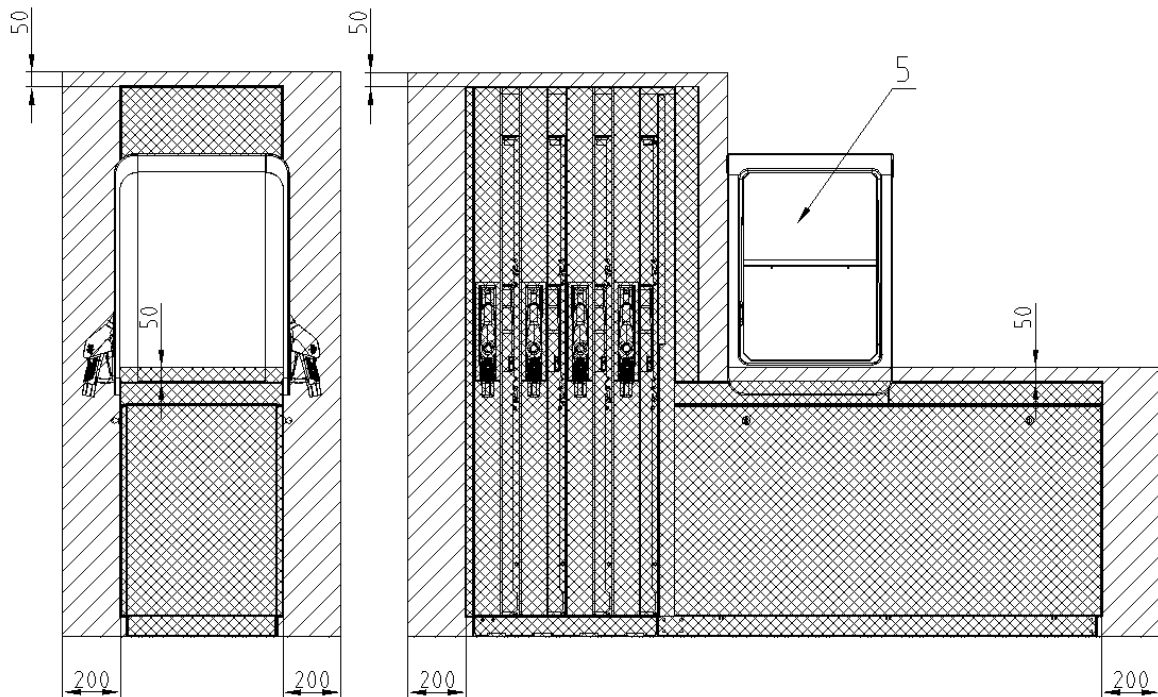
Picture 69 – Example of drawing the danger zones of the OCEAN TOWER dispenser according to EN 13617-1 (5 - non-explosive area)
