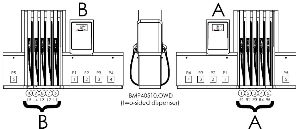
Picture 79 – Example of a standard dispenser with two filling points A and B (two simultaneous deliveries, two main displays; ①, ②, ③ ... - nozzle position in electronic counter)
