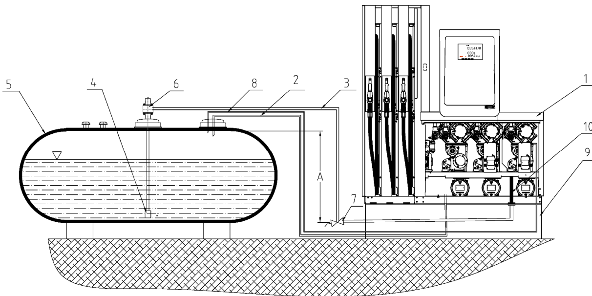
Picture 73 – Example of connection of the dispenser with suction pumps to the aboveground storage tank
