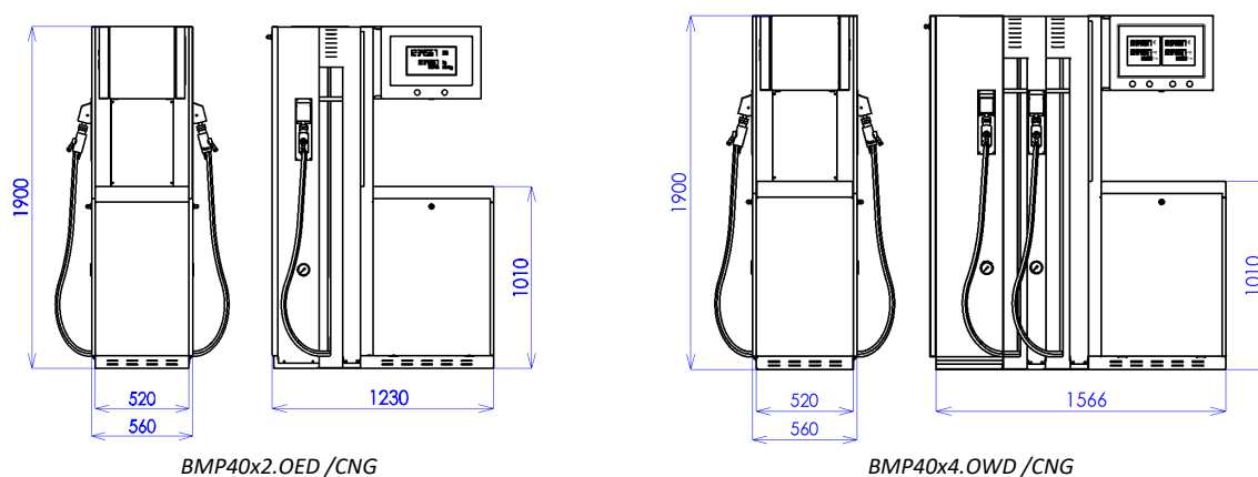
Figure 24 – Overview of standard OCEAN EURO CNG dispensers
