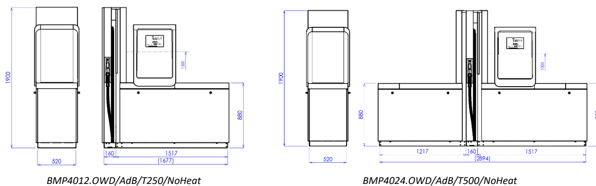
Picture 35 - OCEAN TOWER ADBLUE® dispenser model without internal heating and storage tank 250L or 500L
