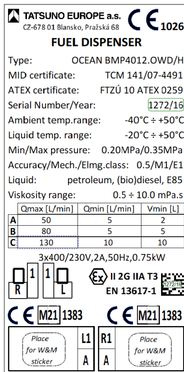
Figure 56 - Nameplate of a two-hose gasoline/diesel dispenser
