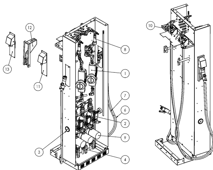
Figure 55 - Basic parts of the CNG dispensing module and its cover
