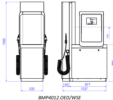
Figure 36 - OCEAN TOWER WSE standard model
