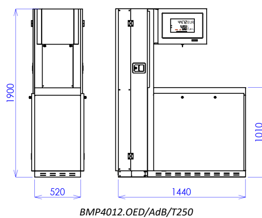
Figure 20 - Model of OCEAN EURO ADBLUE® dispenser with 250L storage tank and pump
