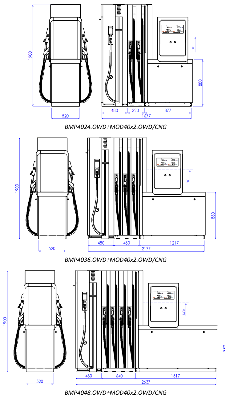
Figure 44 – Overview of OCEAN TOWER COMBI CNG dispensers, x=1,2,3 is the number of the CNG pressure inputs
