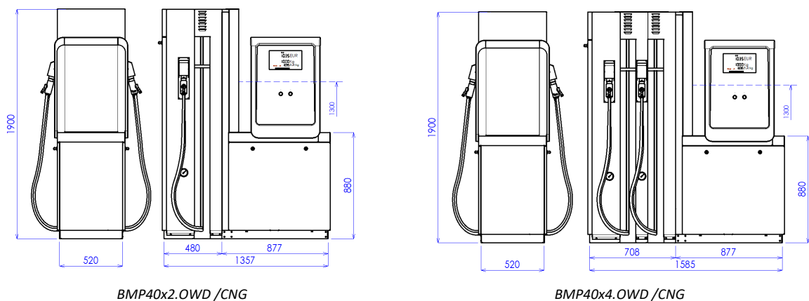
Picture 38 – OCEAN TOWER CNG standard models
