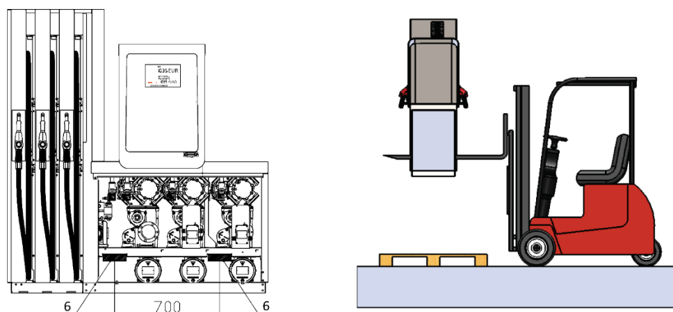
Picture 66 – Lifting the dispenser from the wooden transport pallet
