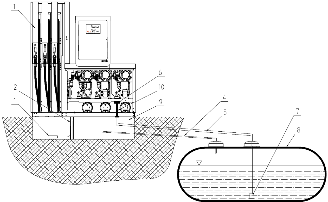
Picture 72– Example of connection of the dispenser with suction pumps to an underground tank
