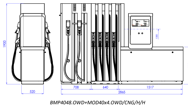
Figure 45 – Example of the OCEAN TOWER COMBI CNG model with four CNG filling hoses for standard and high flow (/H)
