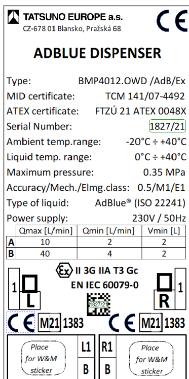
Figure 61 - Nameplate of two-hose AdBlue® dispenser
