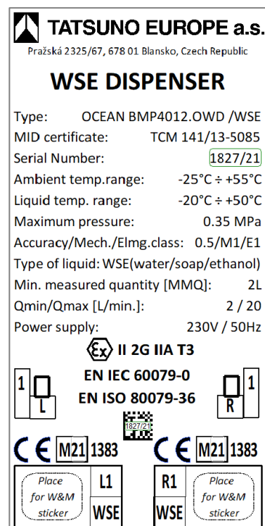
Figure 62 - Nameplate of two-hose WSE dispenser
