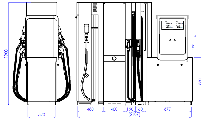
BMP4012.OWD+MOD4012.OWD/LPG+MOD40x2.OWD/CNG
