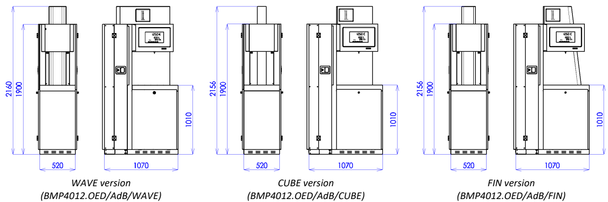
Figure 21 - Design variants of OCEAN EURO /ADB dispensers
