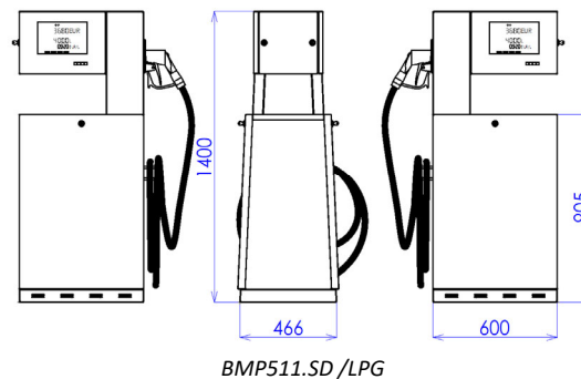
Figure 4 – Standard model SHARK JUNIOR LPG
