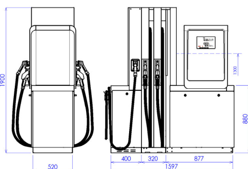
BMP4024.OWD+MOD4012.OWD/LPG
