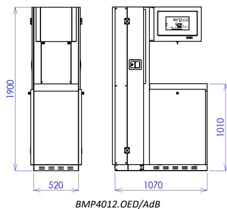
Figure 22 - Overview of standard OCEAN EURO /ADB dispensers
