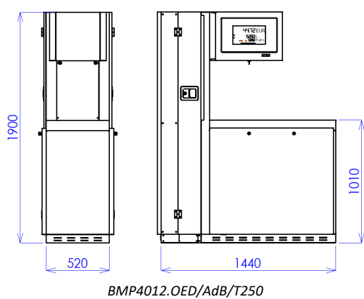
Figure 23 - Model of OCEAN EURO /ADB dispenser with 250L storage tank and pump
