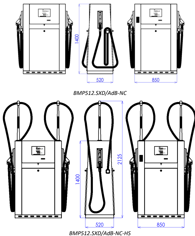
Figure 11 - Standard SHARK ECONOMY /ADB models (non-simultaneous deliveries „-NC“)
