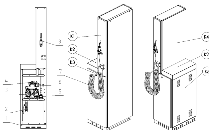
Figure 58 - Basic parts of the WSE dispensing module and its cover
