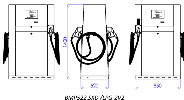
Figure 9 – Standard SHARK ECONOMY LPG models
