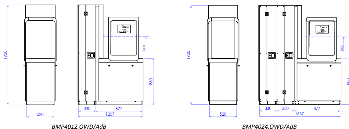
Figure 35 – OCEAN TOWER /ADB standard model with internal heating
