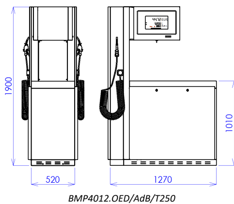
Figure 26 - Model of OCEAN EURO /ADB dispenser with 250L storage tank and pump
