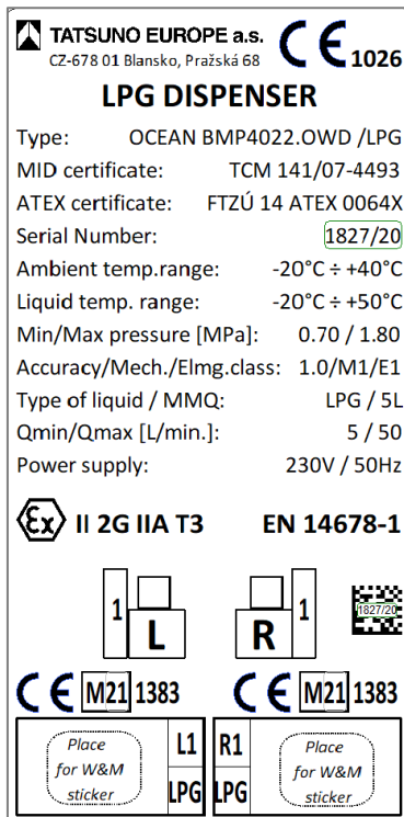
Figure 64 - Nameplate of two-hose LPG dispenser
