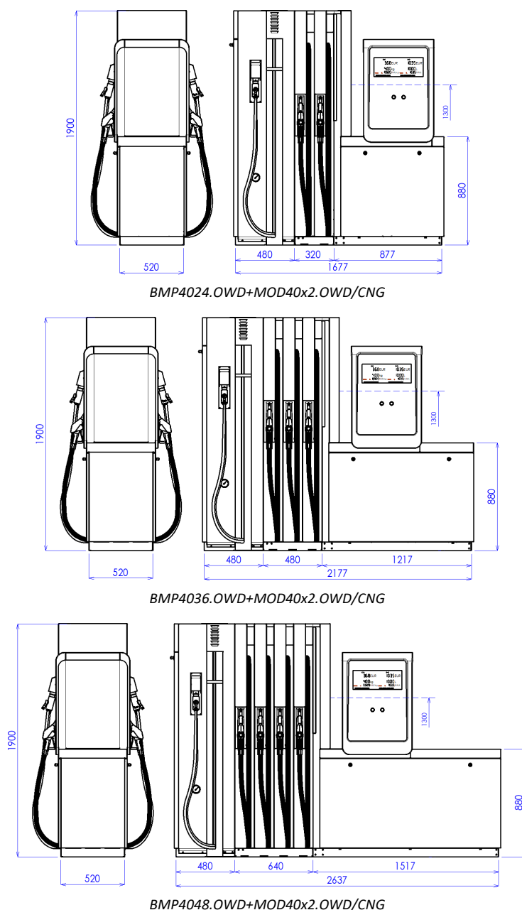
Figure 47 – Overview of OCEAN TOWER COMBI CNG dispensers, x=1,2,3 is the number of the CNG pressure inputs
