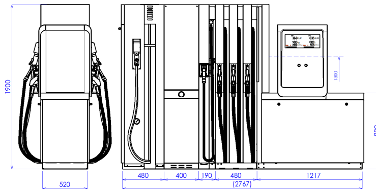
BMP4036.OWD+MOD4012.OWD/LPG+MOD40x2.OWD/CNG
