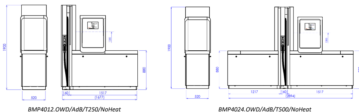
Picture 38 - OCEAN TOWER /ADB dispenser model without internal heating and storage tank 250L or 500L
