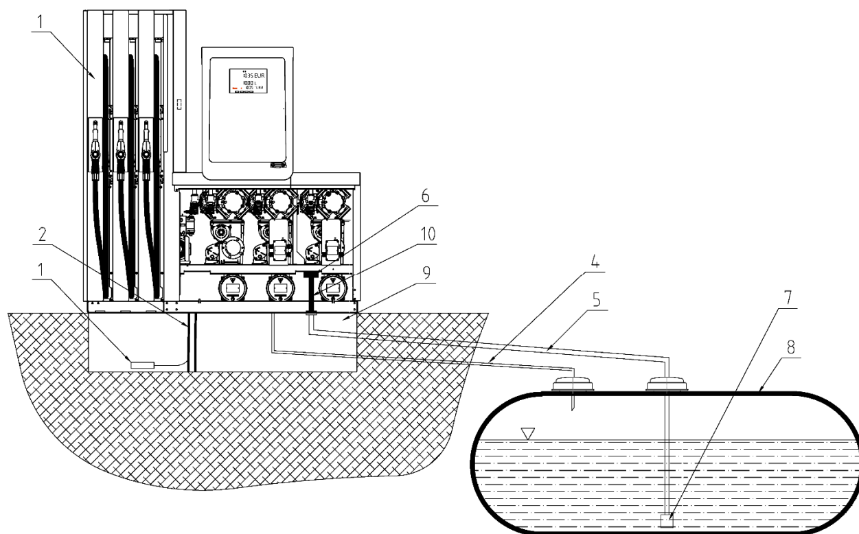
Picture 76– Example of connection of the dispenser with suction pumps to an underground tank
