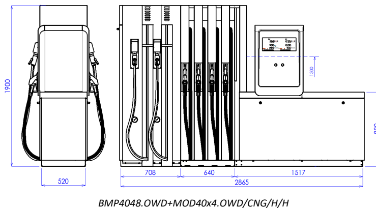
Figure 48 – Example of the OCEAN TOWER COMBI model with four CNG filling hoses for standard and high flow (/H)
