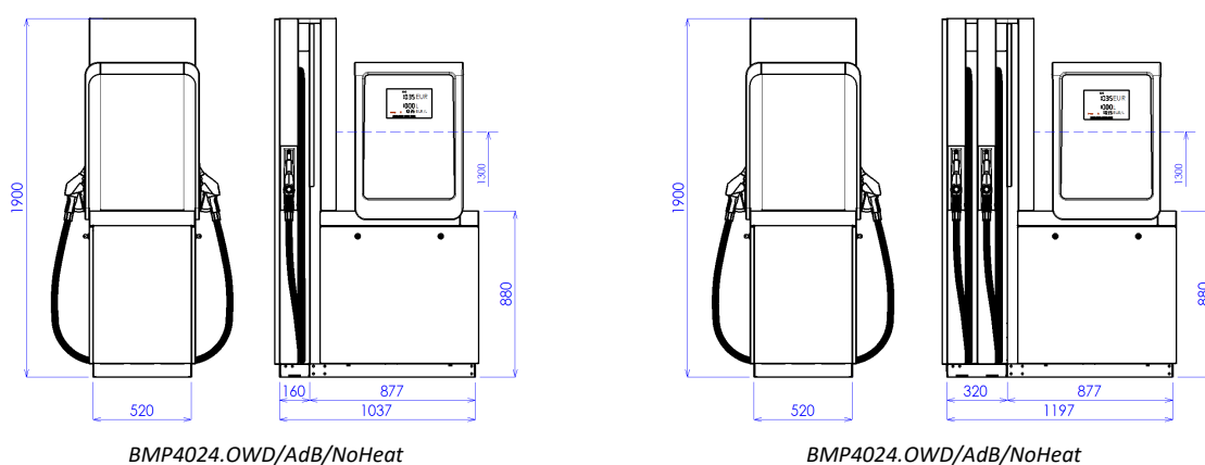
Figure 36 - OCEAN TOWER /ADB dispenser model without internal heating
