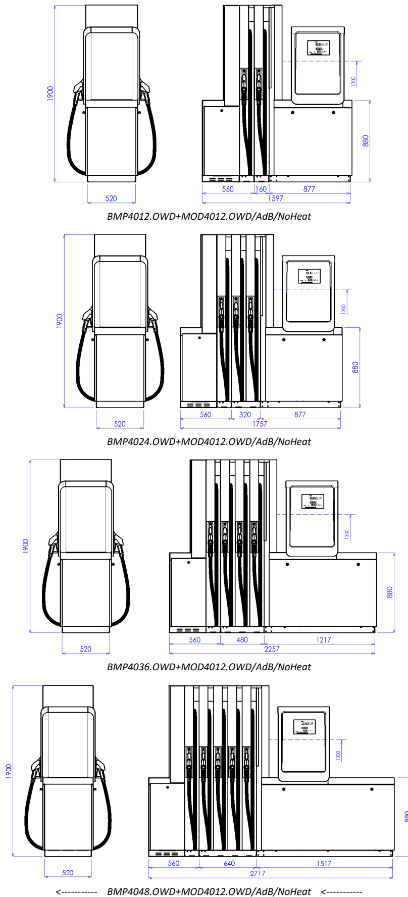
Figure 45 – Overview of OCEAN TOWER COMBI ADB dispensers with AdBlue module without heating (for temperatures from 0°C to 40°C).
