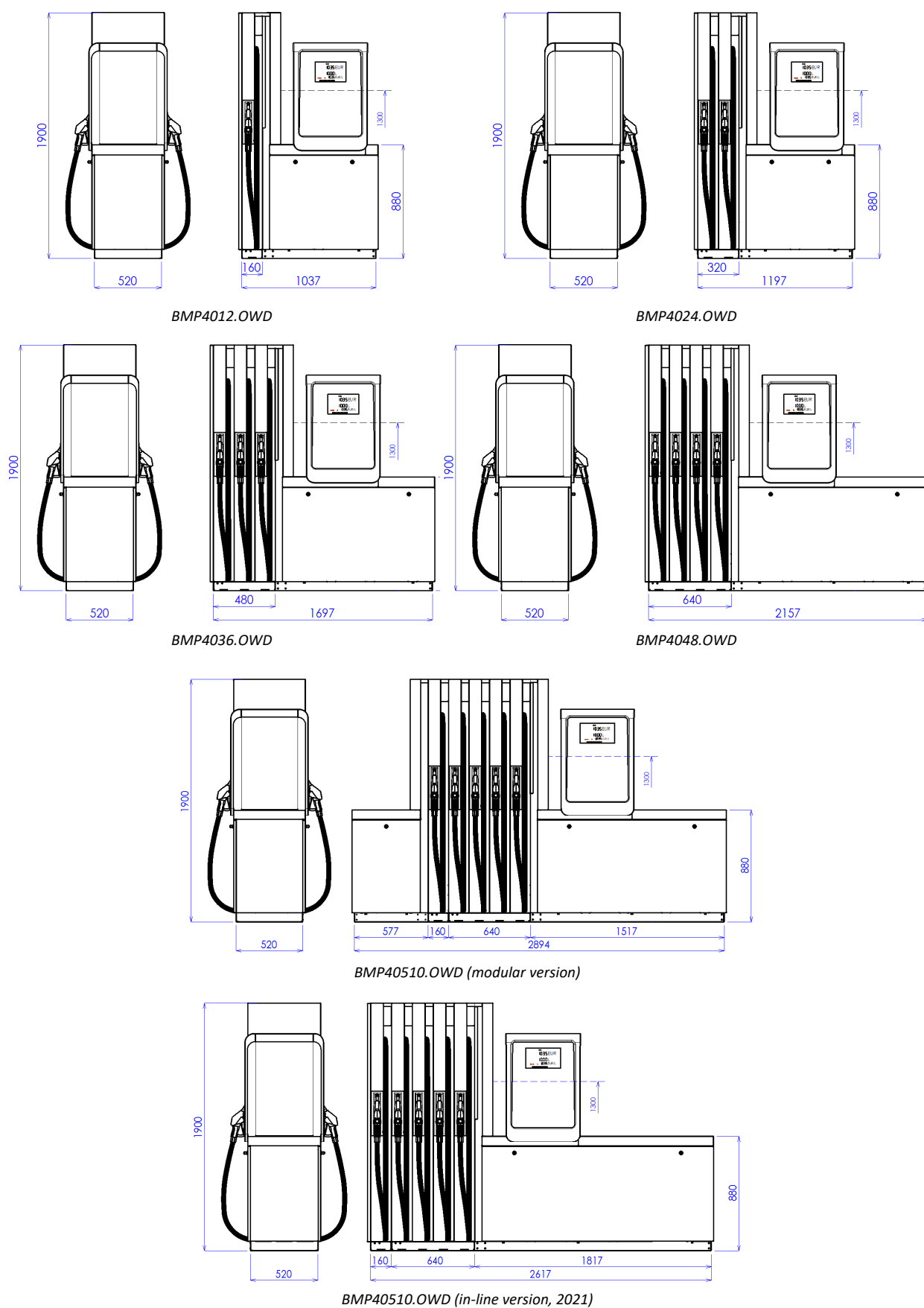
Figure 31 - Overview of standard OCEAN TOWER models
