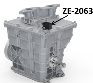
Picture 90 – Pumping monoblock FP-1022 (MVP-X) with air flow sensor ZE-2063
