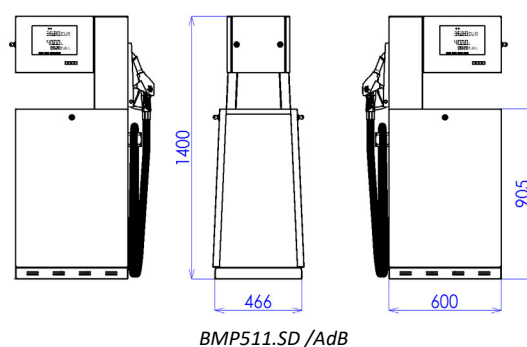
Figure 5 - Standard SHARK JUNIOR /ADB dispenser models with nozzles positioned at the front (-ZV2)
