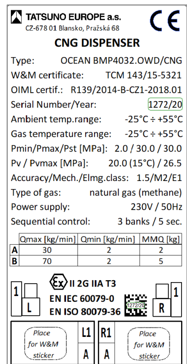
Figure 67 - Nameplate of two-hose CNG dispenser
