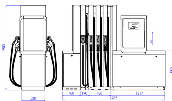
BMP4036.OWD+MOD4012.OWD/LPG-HR
