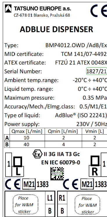
Figure 65 - Nameplate of two-hose AdBlue® dispenser
