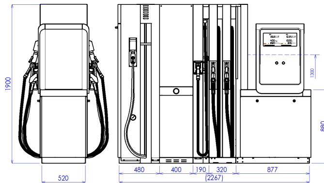
BMP4024.OWD+MOD4012.OWD/LPG+MOD40x2.OWD/CNG
