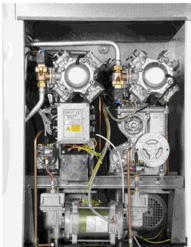
Figure 93 - Uncovered dispenser, side B
