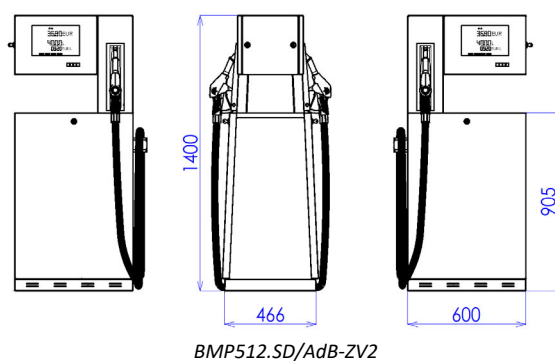
Figure 5 - Standard SHARK JUNIOR /ADB dispenser models with nozzles positioned at the front (-ZV2)
