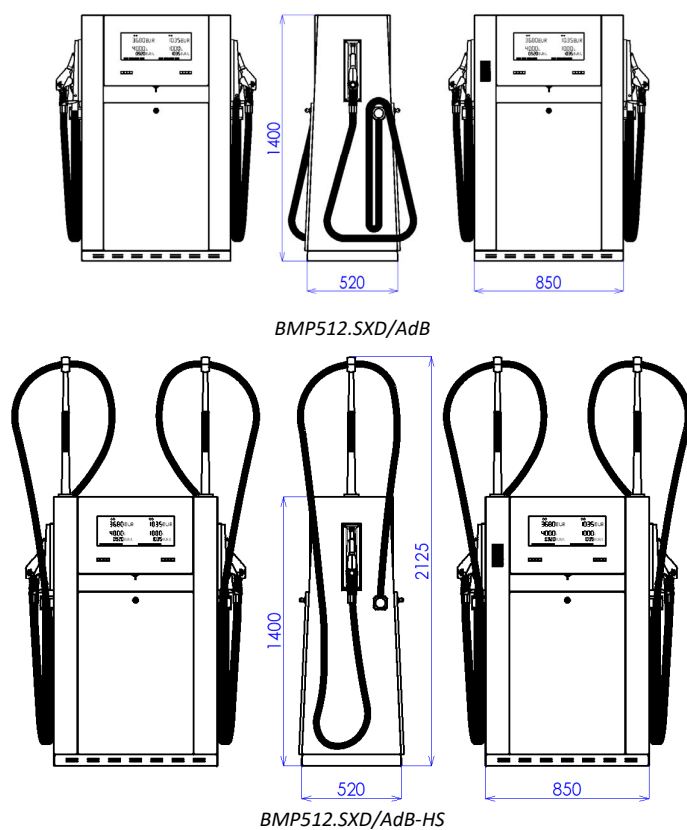
Figure 10 - Standard SHARK ECONOMY /ADB models (two simultaneous deliveries)
