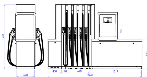
BMP4048.OWD+MOD4012.OWD/LPG-HR
