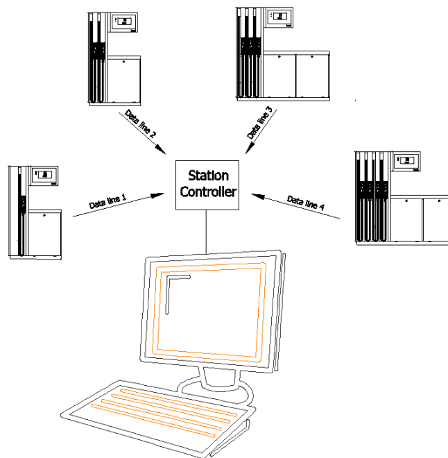
Figure 81 – Radial data line from dispensers
