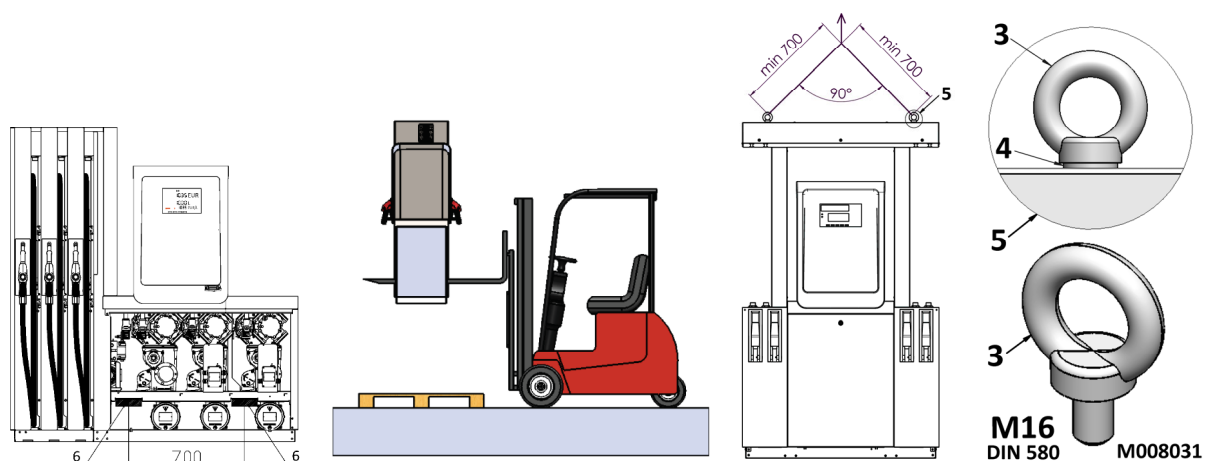
Picture 70 – Lifting the dispenser from the wooden transport pallet
