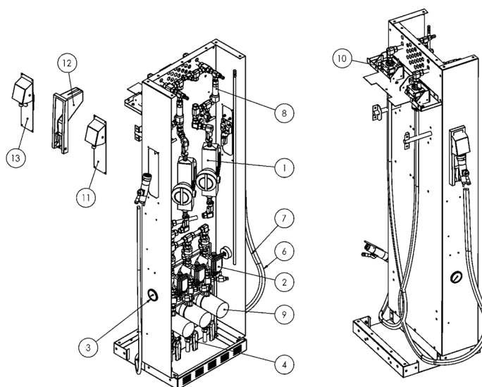
Figure 59 - Basic parts of the CNG dispensing module and its cover
