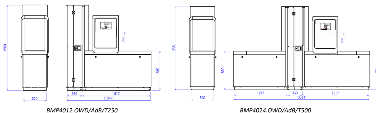
Picture 37 - OCEAN TOWER /ADB dispenser model with internal heating and storage tank 250L or 500L
