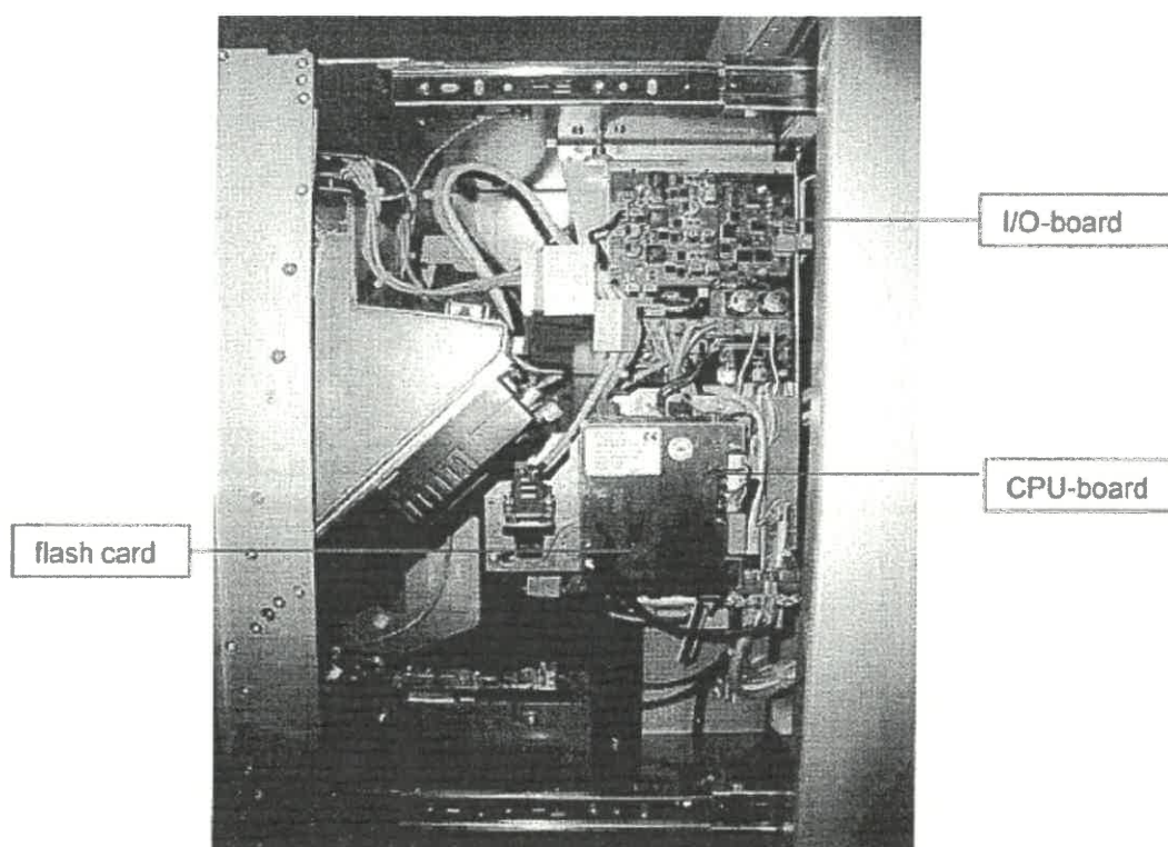
Picture No. 13: Sealing of the CPU and flash card of Hectronic GmbH HECSTAR/ HECFLEET NT self-service device
