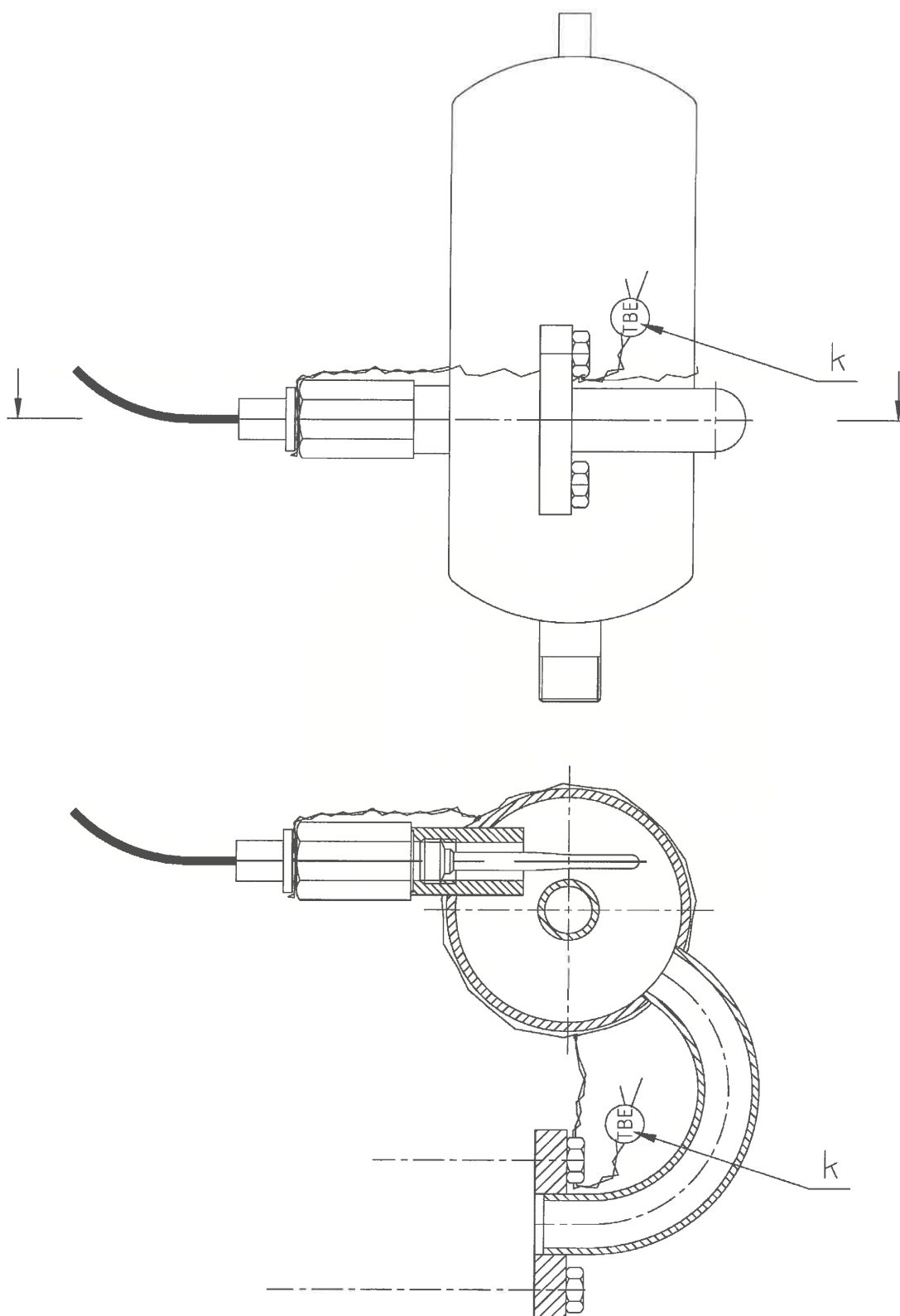
Picture No. 8: Sealing of the Pt100 in gas separator
