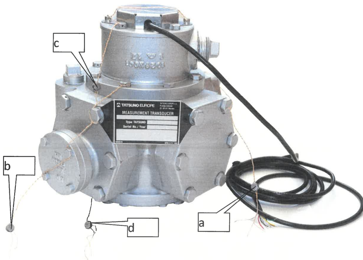
Picture No. 2b: Sealing of the FM-1029 measurement transducer
