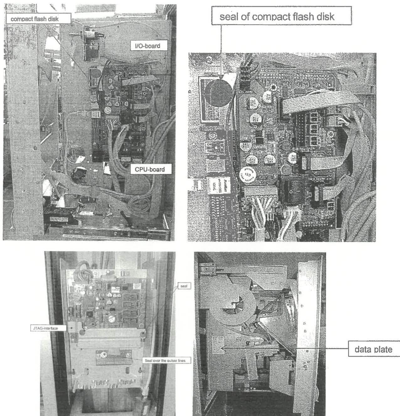
Picture No. 20: Sealing of CPU, type label, flash disk and pulsers of Hectronic GmbH HECONOMY self-service device
