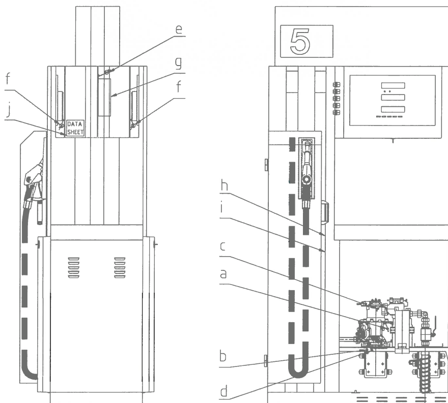
Picture No. 1a: The sealing of OCEAN BMP 4xxx.O/AdB AdBlue dispenser, version EURO
