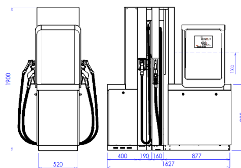
BMP4012.OWD+MOD4012.OWD/LPG-HR
