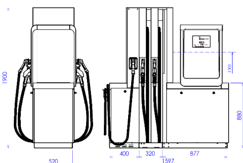
BMP4024.OWD+MOD4012.OWD/LPG
