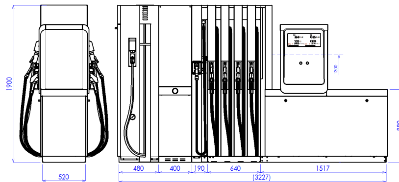
BMP4048.OWD+MOD4012.OWD/LPG+MOD40x2.OWD/CNG
