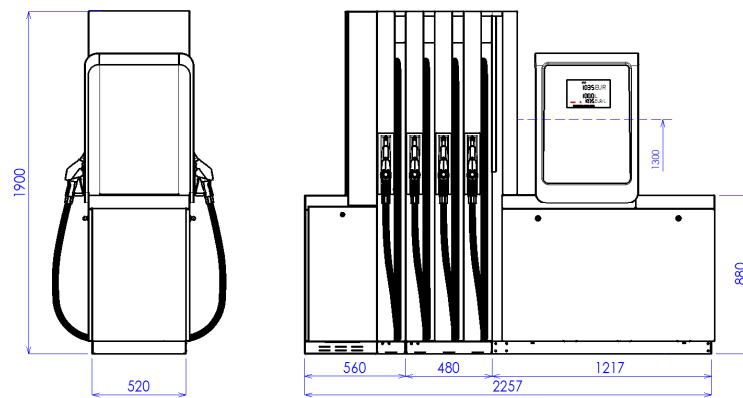
BMP4036.OWD+MOD4012.OWD/AdB/NoHeat
