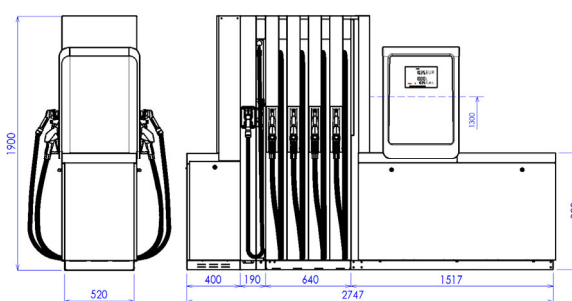
BMP4048.OWD+MOD4012.OWD/LPG-HR
