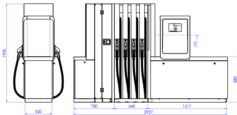
----- BMP4048.OWD+MOD4012.OWD/AdB -----
