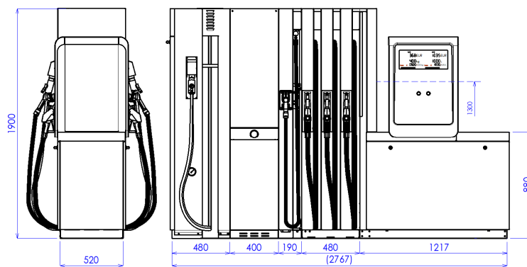
BMP4036.OWD+MOD4012.OWD/LPG+MOD40x2.OWD/CNG
