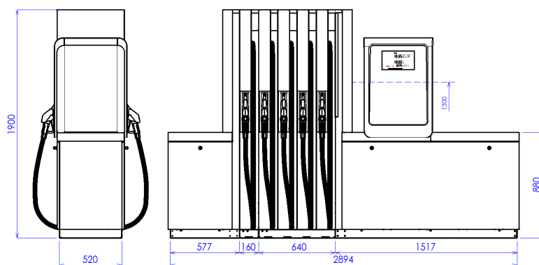
BMP4048.OWD
