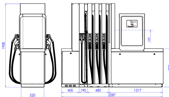
BMP4036.OWD+MOD4012.OWD/LPG-HR
