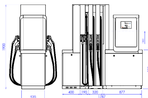
BMP4024.OWD+MOD4012.OWD/LPG-HR
