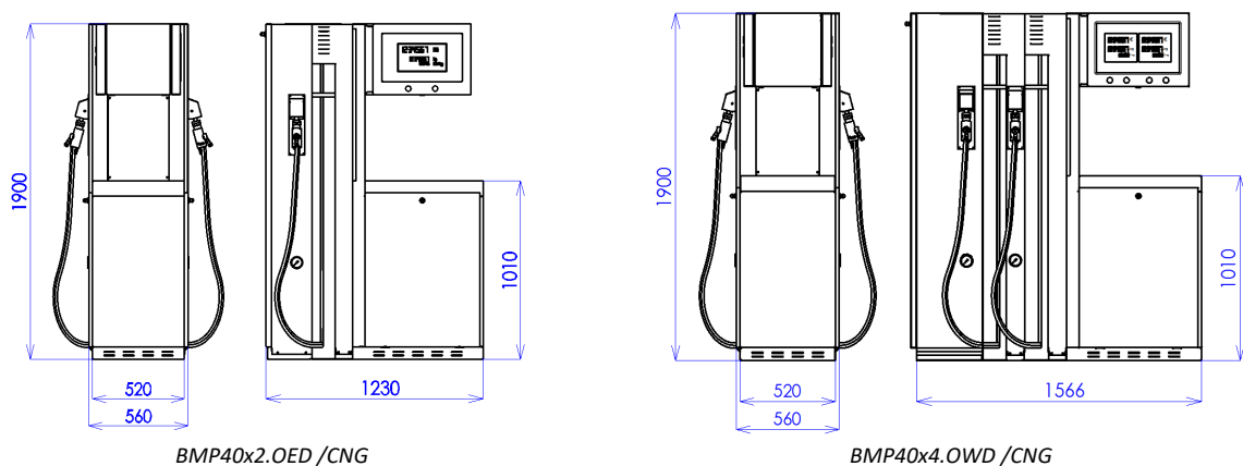
Figure 27 – Overview of standard OCEAN EURO CNG dispensers
