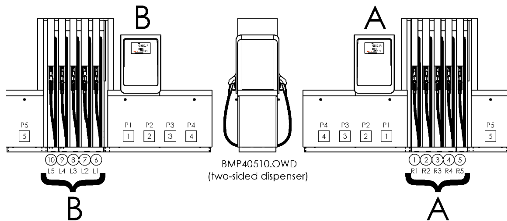
Picture 84 – Example of a standard dispenser with two filling points A and B (two simultaneous deliveries, two main displays; ①, ②, ③ ... - nozzle position in electronic counter)
