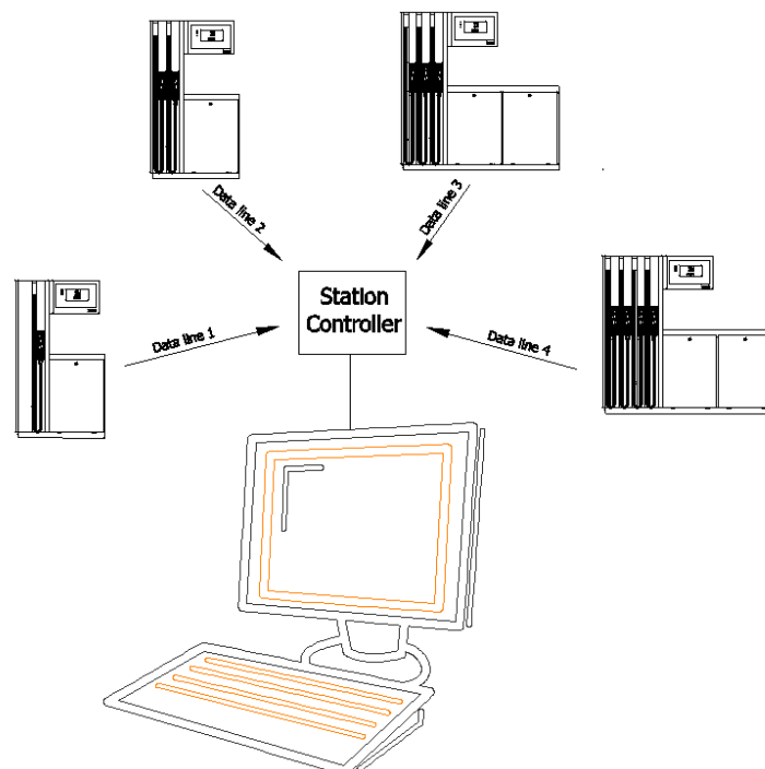
Figure 81 – Radial data line from dispensers
