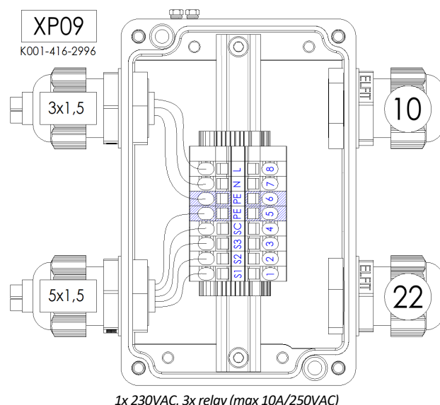
1x 230VAC, 3x relay (max 10A/250VAC)
