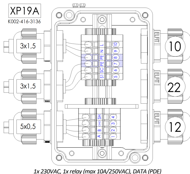
1x 230VAC, 1x relay (max 10A/250VAC), DATA (PDE)
