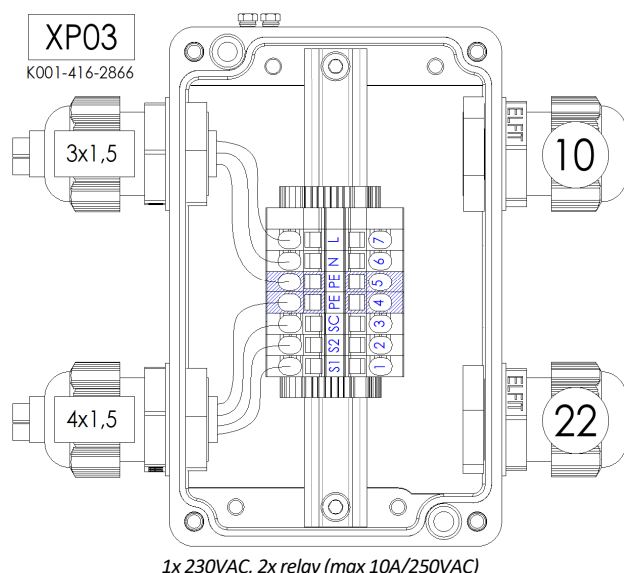
1x 230VAC, 2x relay (max 10A/250VAC)
