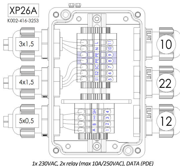
1x 230VAC, 2x relay (max 10A/250VAC), DATA (PDE)
