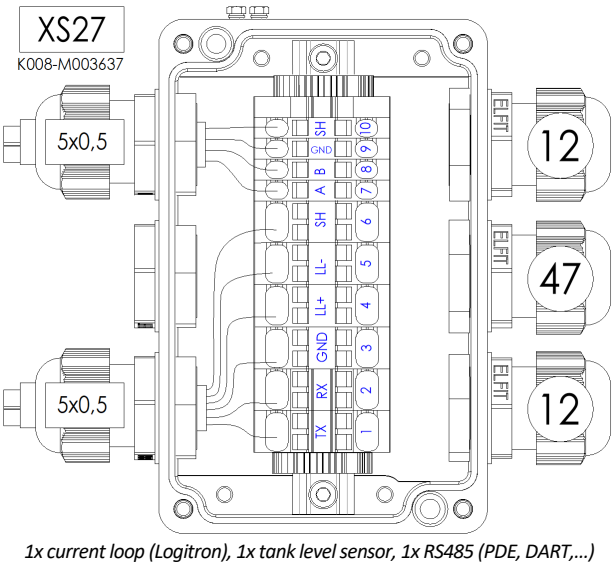
1x current loop (Logitron), 1x tank level sensor, 1x RS485 (PDE, DART,...)
